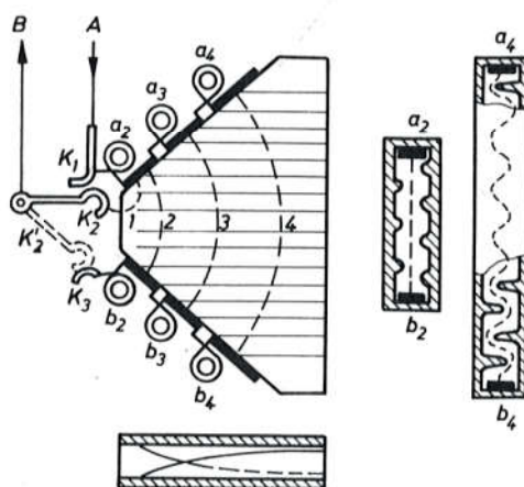
Sl. 760. Keramička komora s valovitim rasporom (General Electric)
