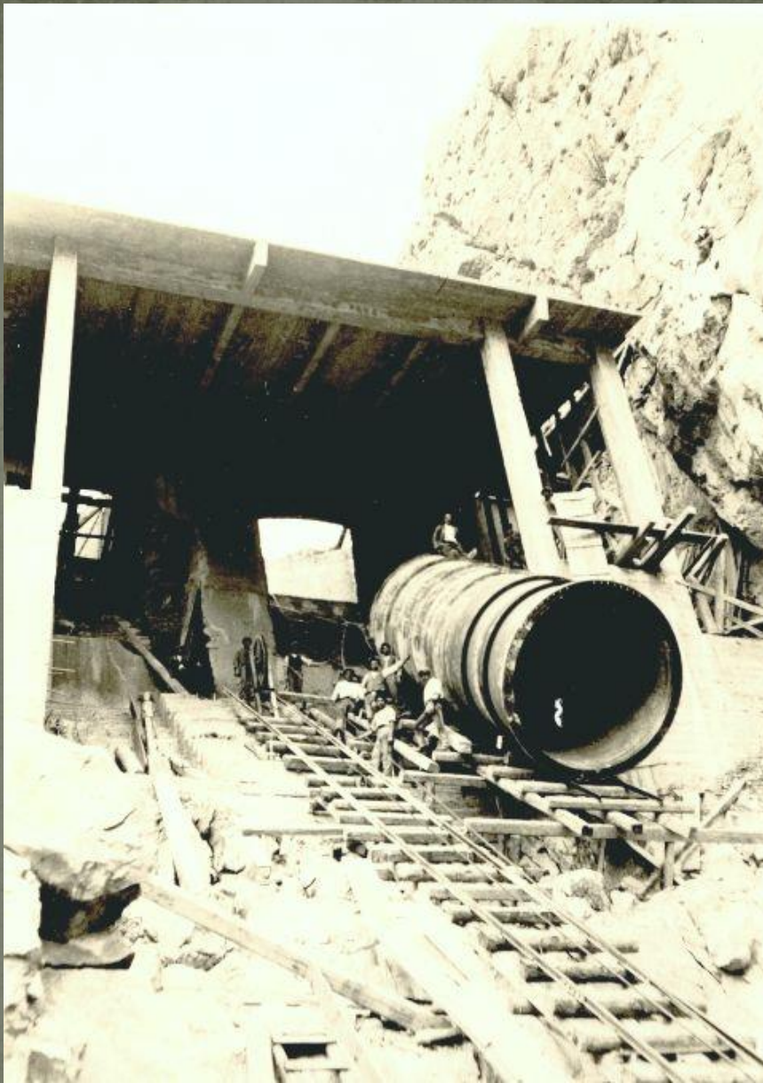
Transportation of the penstock parts to the surge chamber
