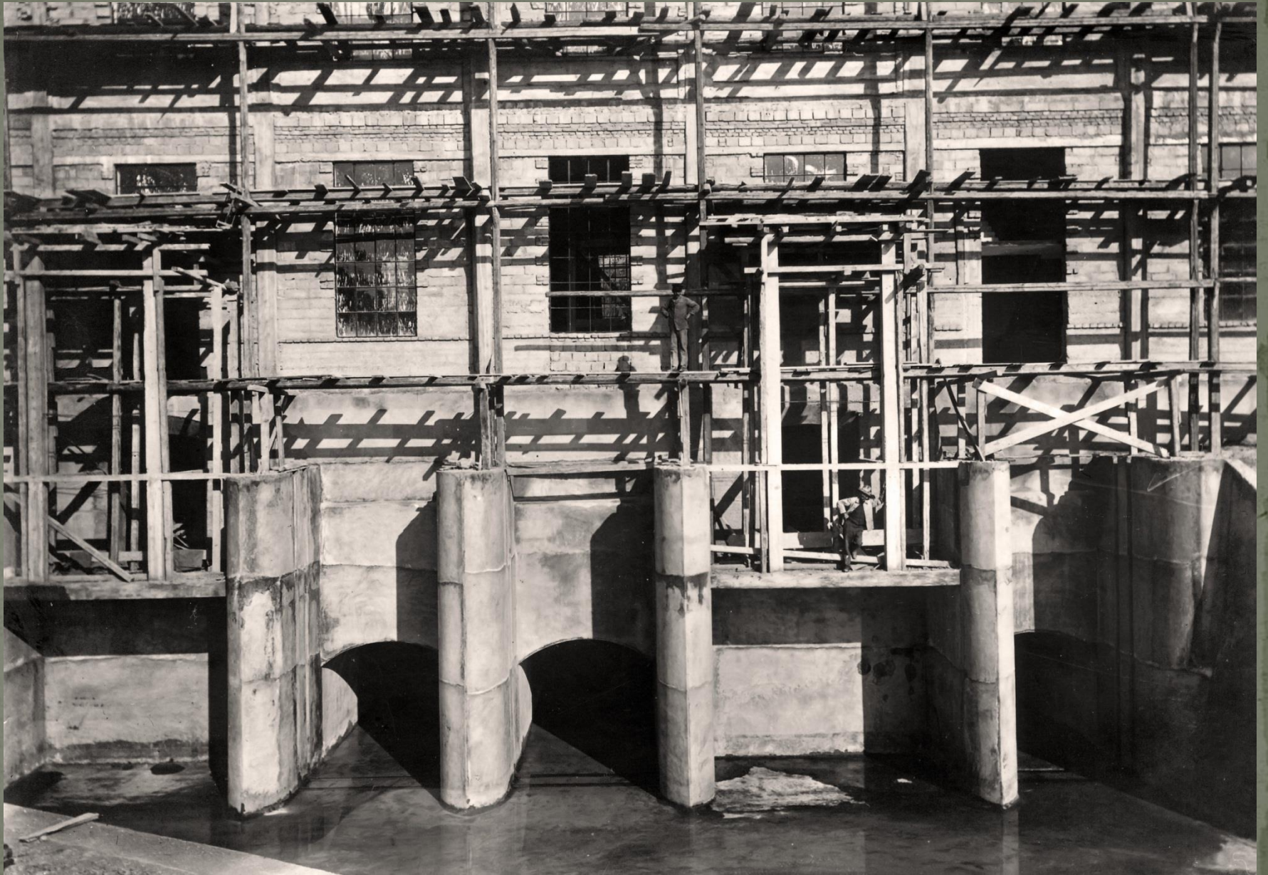
Final construction works of the first stage
