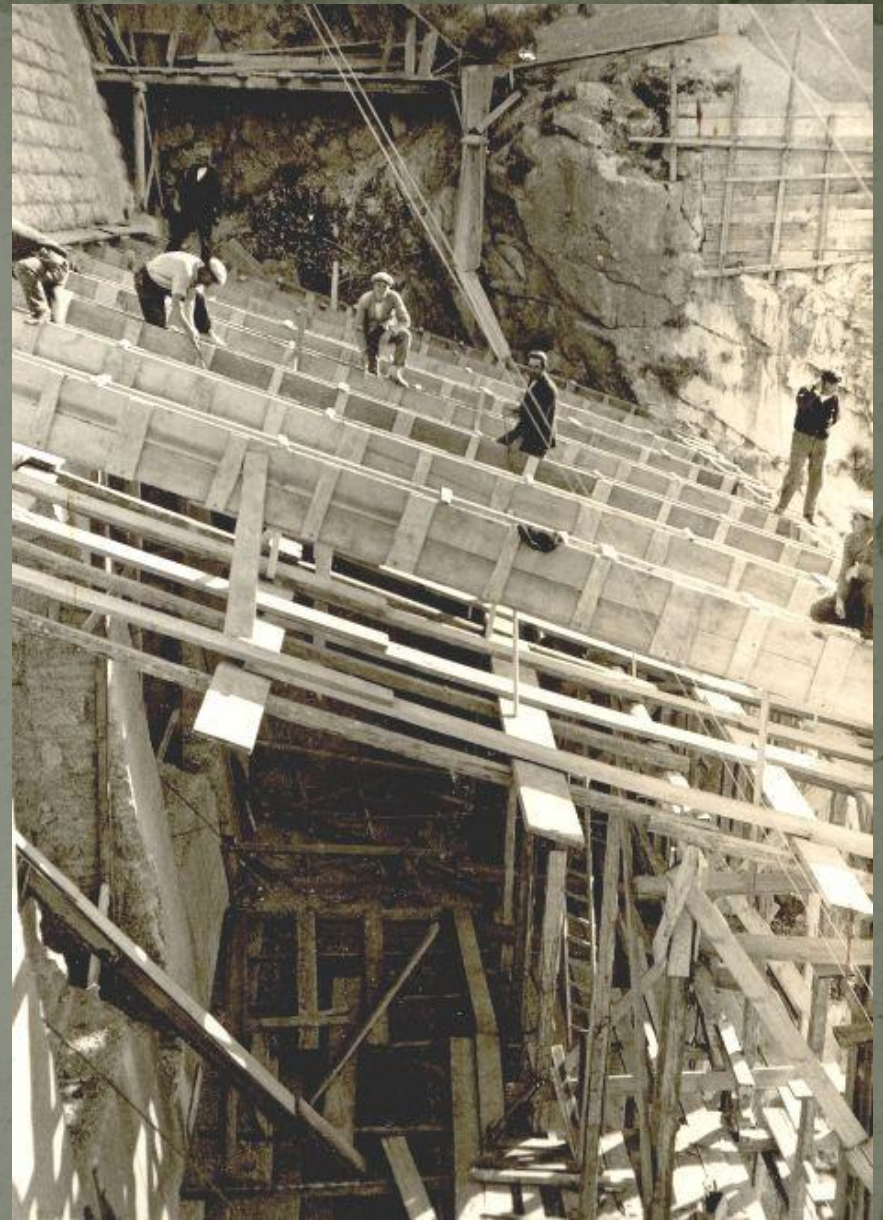
Final works in the valve chamber
