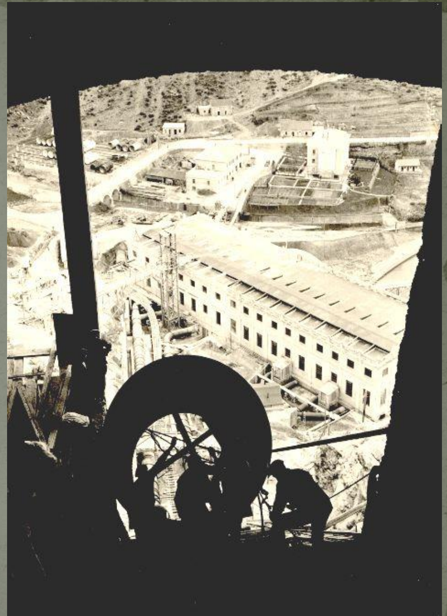
Transportation of the penstock parts to the surge chamber
