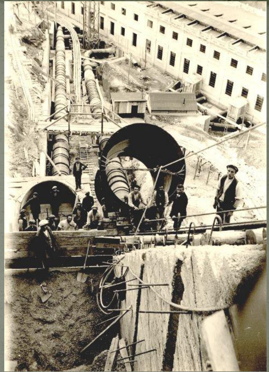
A cable railway for transportation of the penstock parts was constructed
