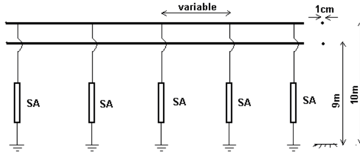
Figure 1 – Line geometry adopted in the calculations.
