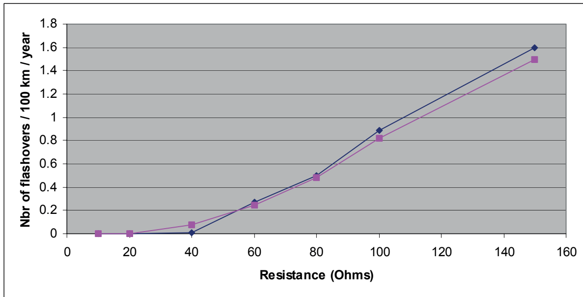
Figure 4 : Multiphase flashover rate of circuit 2 not equipped with line arrester when both external phases of circuit 1 are protected by line arresters (gapped arresters -■-, gapless arresters -◆-).
