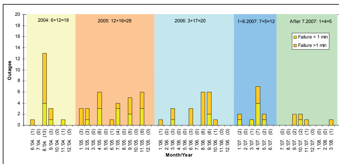
Figure 5-Review of outages on line 110 kV Ston-Komolac (before and after LSA application) (2007: 1-6 without LSA (blue), 2007: 1-12/2008:1-3 with LSA (green))
