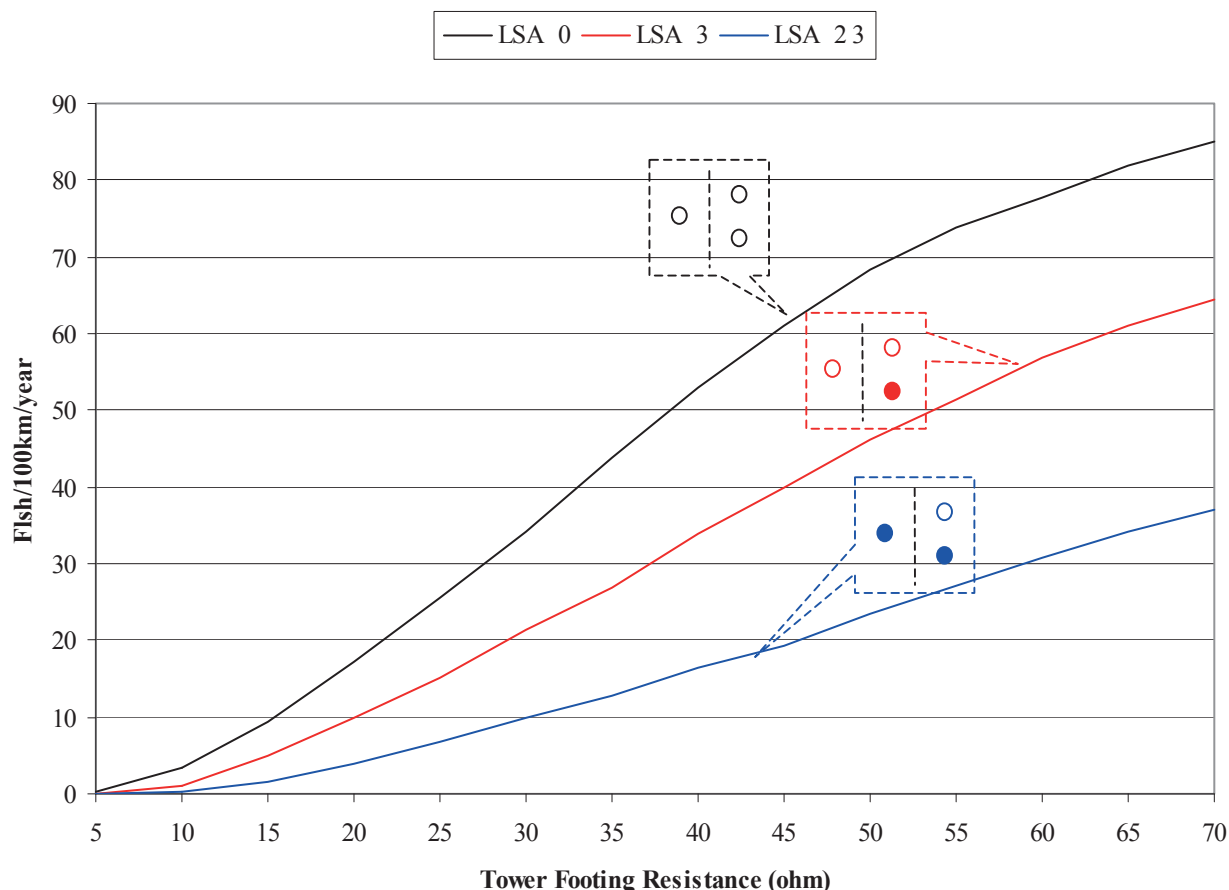
Figure 2 - Line lightning performance for different tower footing resistances and different LSA installation configurations
