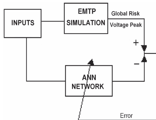
Fig. 2. Supervised learning of ANN.
