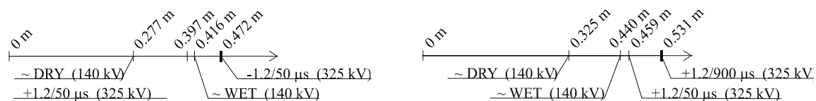
Figure 16. Flashover clearing distance l_{ad} at the insulator and between two phases with regard to the insulation level U_m = 72,5 kV (140/325 kV).
