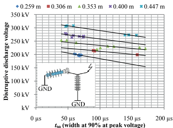
Figure 13: Voltage and shape dependency on discharge
