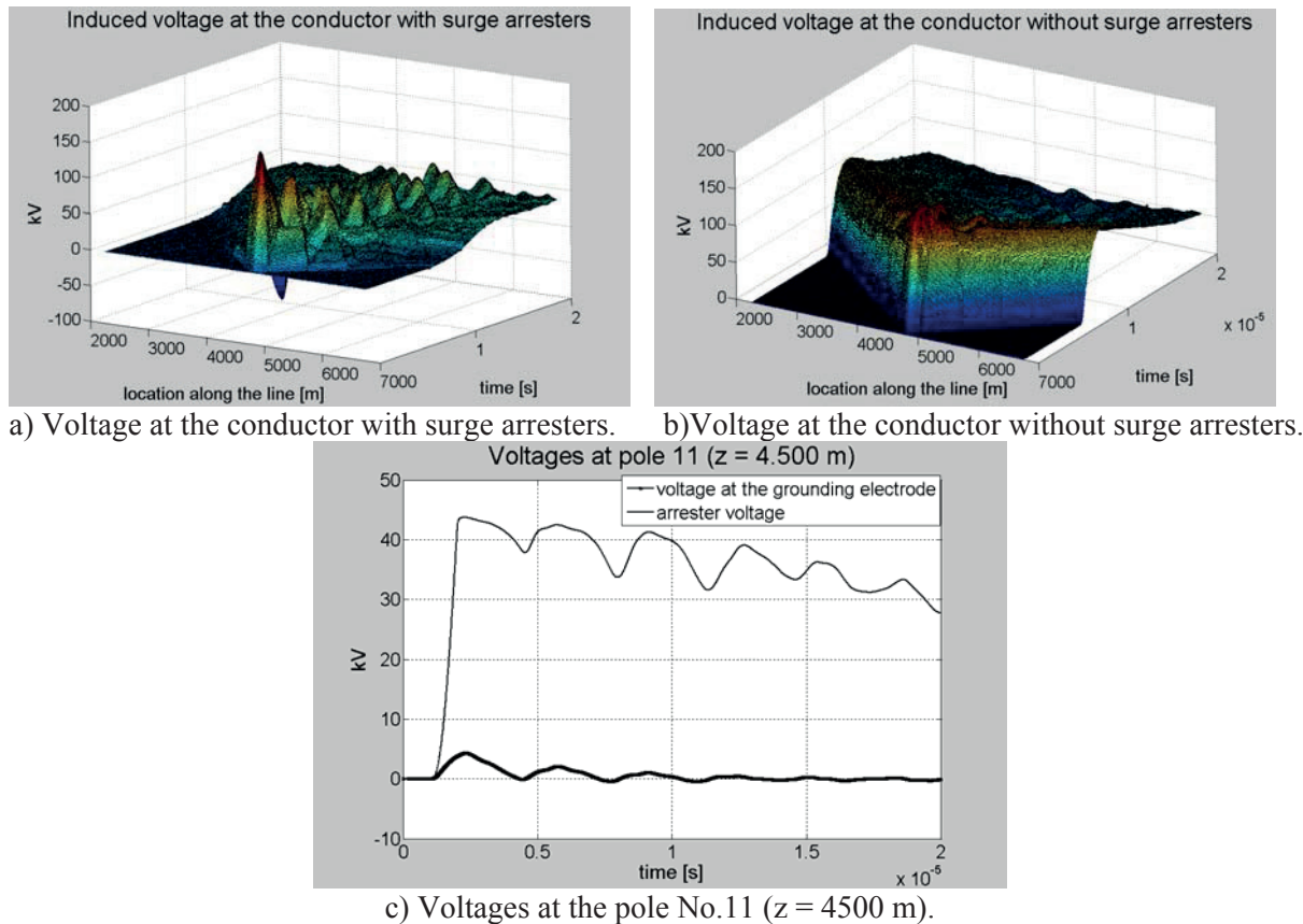
Figure 4– Voltages along a line with surge arresters each 450 m ( R_g = 10 \text{ Ohms} ), produced by a 45 kA lightning discharge ( 2 \times 40 \text{ } \mu\text{s} ), propagating with a velocity v = 0.1 c , that strikes at z = 4800 \text{ m} , at a distance of 70 m from the line.
