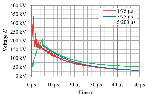
Figure 5: Phase B overvoltages for variable t_f – samples ( I_1 = 40 kA, R_g = 10 Ω, line voltage is 0 kV)
