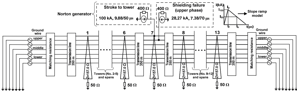
Figure 2. – Model of 220 kV double-circuit line
