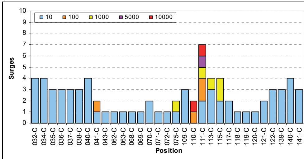
Figure 7- Review of LSA surges registered by Excount II monitoring sensors in Phase L3 (C)
