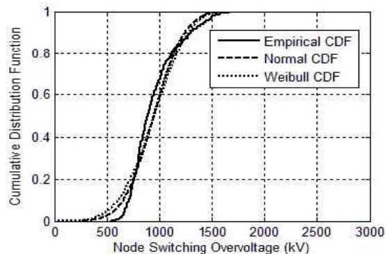
Fig. 4. Cumulative distribution of overvoltages.
