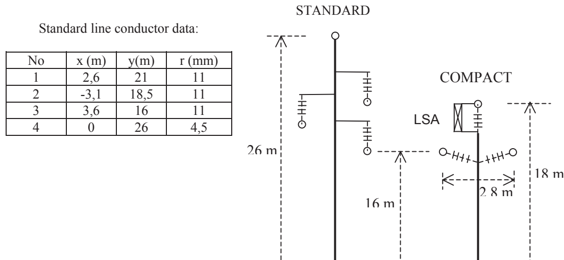
Figure 1 - “Standard” shielded and Compact unshielded single circuit line designs
