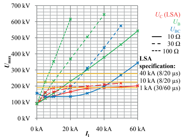
Figure 4: Maximum U_{\max}(I_l, R_g, 5/75 \mu s) with respect to 110 kV
