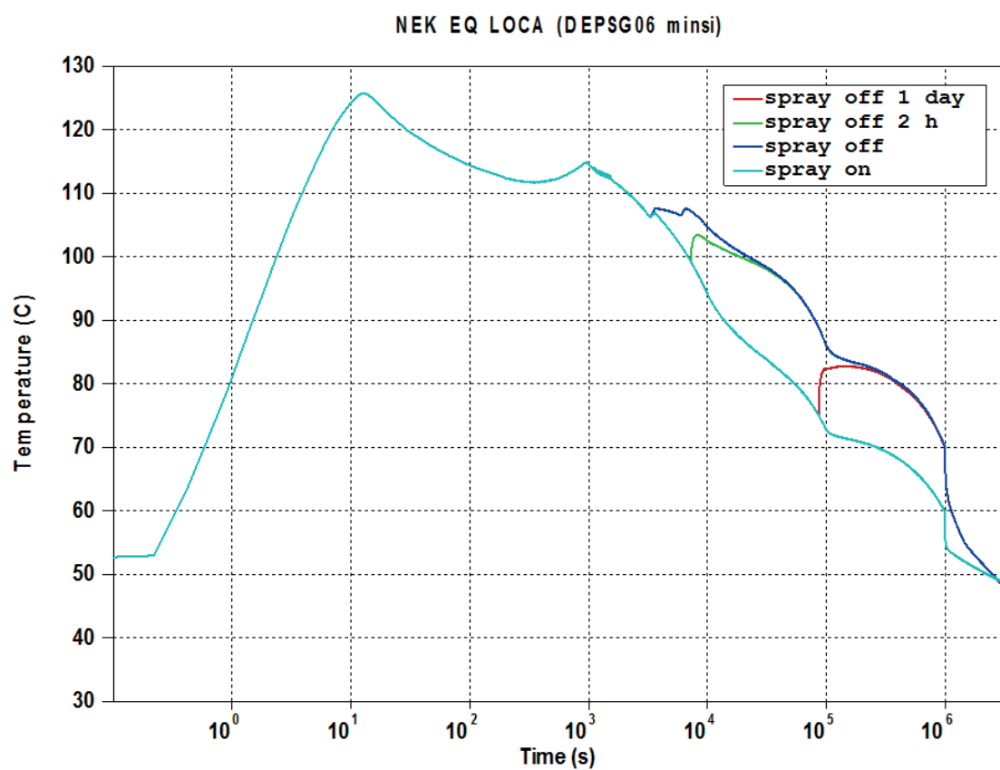
Figure 9: Temperature in containment, EQ LOCA
