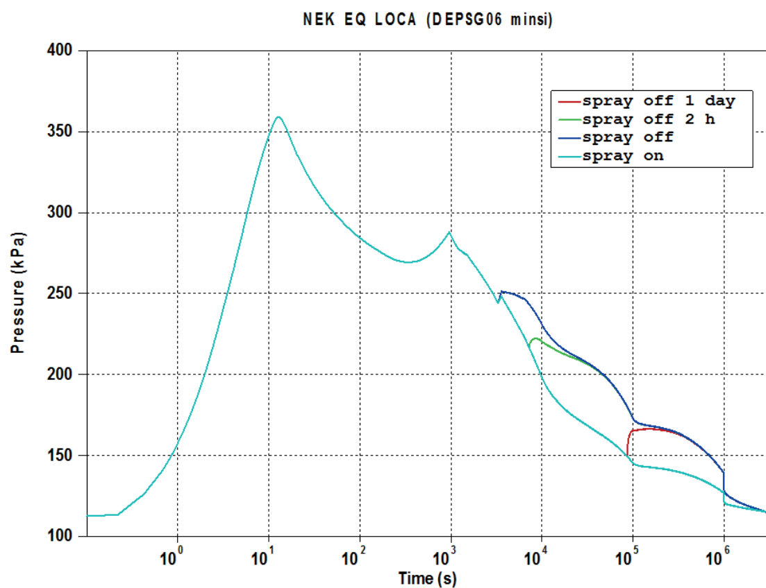
Figure 8: Pressure in containment, EQ LOCA
