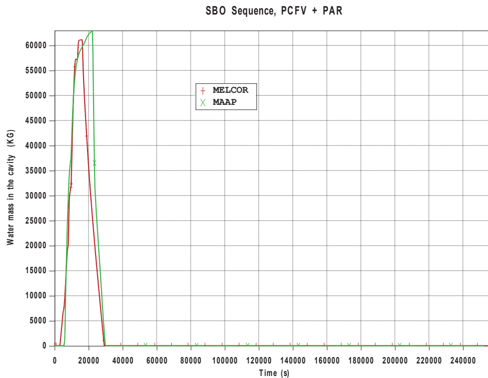
Figure 8: Mass of water in the reactor cavity
