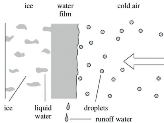
Figure 12 – Wet growth [5]
