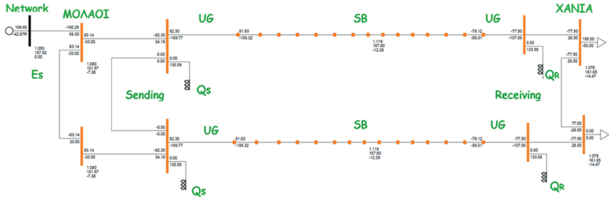
Figure 4. Interconnector model
