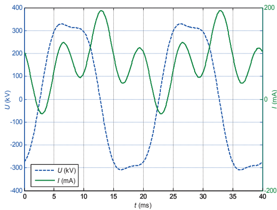
Figure 13. U - I waveforms for U_p=248.6 kV ( I_{DC}=80 mA)
