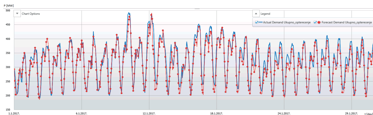
Figure 6 Comparison graph of Actual and Forecast Load Values for Elektrodalmacija Split Distribution in January 2017
