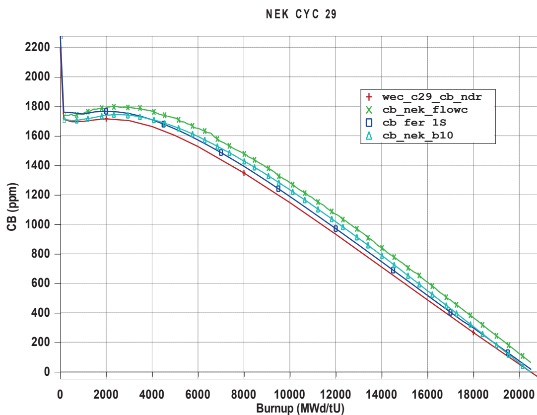
Figure 3 Critical boron concentration depending on burnup
