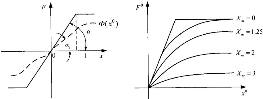
Figure 7.2: (a) Nonlinear static characteristic and (b) smoothed static characteristic of saturation.
