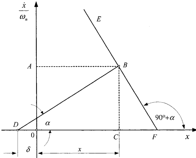
Figure 5.12: Construction of phase trajectory by \delta -method.
