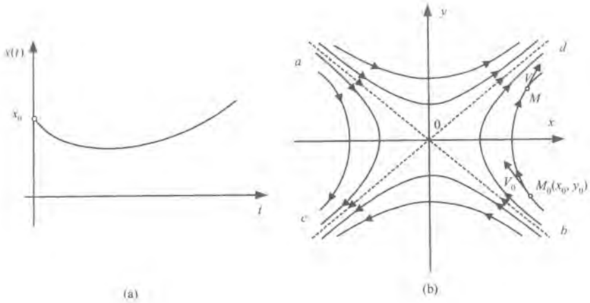
Figure 5.7: Possible form of phase trajectory (a) and phase portrait (b) for linear system with singular point of type saddle.
