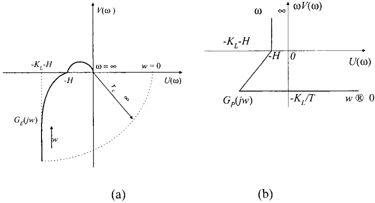
Figure 2.38: Magnified frequency characteristic (a) equivalent G_E(j\omega) and (b) Popov G_P(j\omega) .
