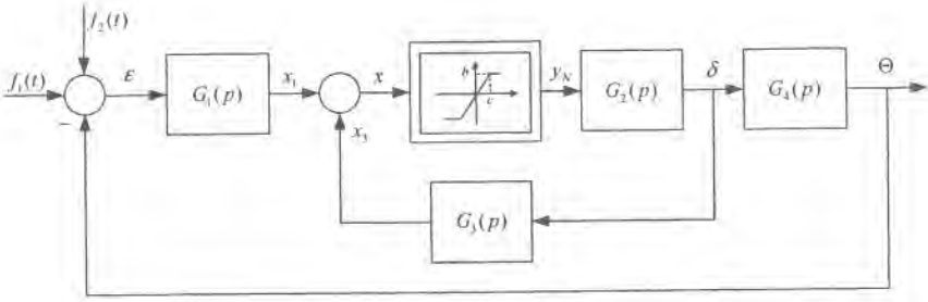
Figure 7.7: Block diagram of the aircraft pitch control system.
