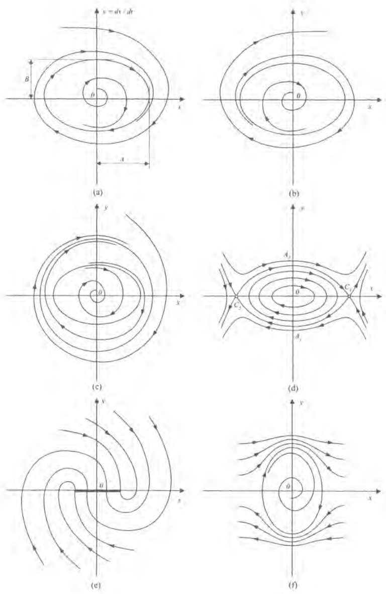
Figure 5.9: The types of phase portraits of nonlinear systems.
