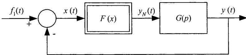
Figure 2.39: Block diagram of forced nonlinear system.
