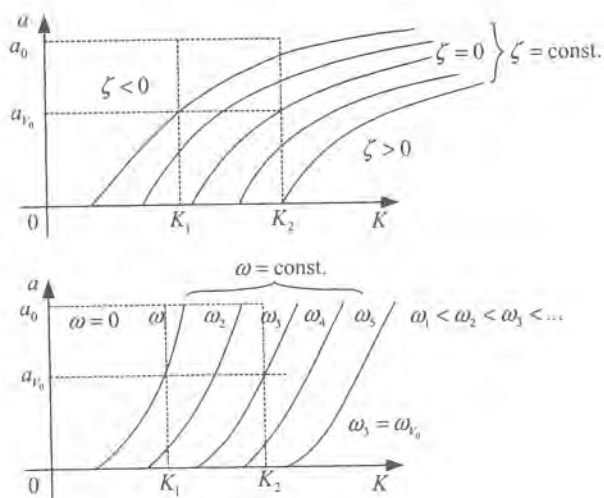
Figure 8.4: Diagrams of performance indicators for transient response of nonlinear control system.
