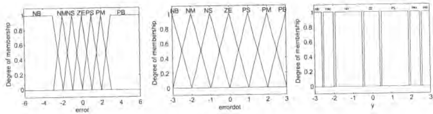
Figure 9.22: Membership functions of the fuzzy regulator. (a) proportional input membership function, (b) derivative output membership function, (c) output membership function.
