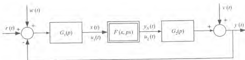
Figure 1.1: Block diagram of a nonlinear system.
