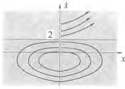
Figure 2.1: Phase trajectories for system (2.1).
