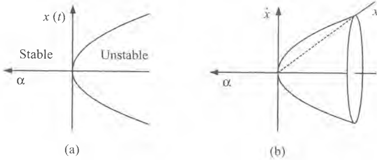
Figure 1.7: Fork bifurcation (a) and Hopf bifurcation (b).
