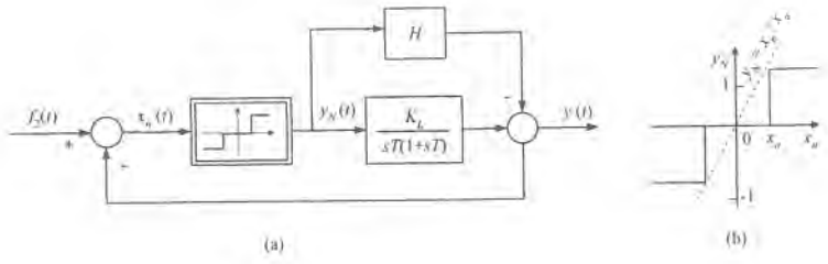
Figure 2.37: Equivalent structure (a) and equivalent nonlinear characteristic (b) for Example 2.22.
