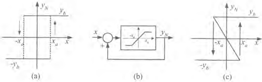
Figure 1.22: Static characteristics of a two-position relay with hysteresis.
