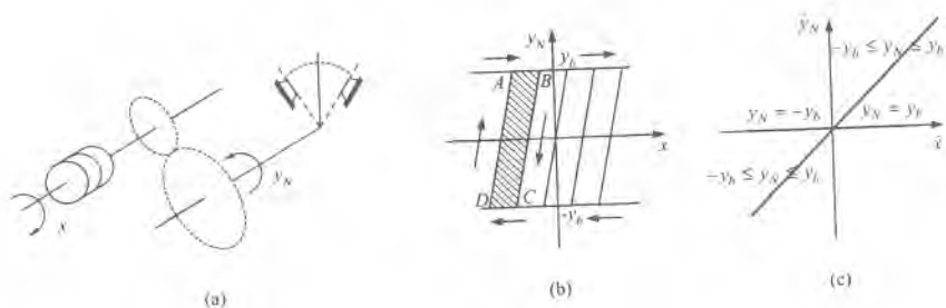
Figure 1.26: Static characteristics of a nonlinear stop-type element.
