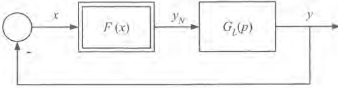
Figure 2.13: Block diagram of a nonlinear system.
