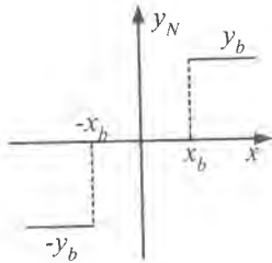
Figure 1.19: Static characteristic of a two-position polarized relay without hysteresis.
