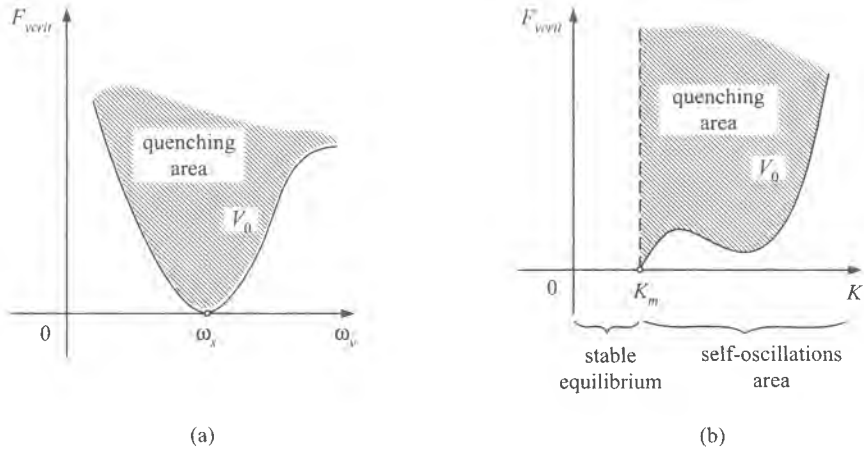
Figure 6.22: Typical forms of quenching areas.
