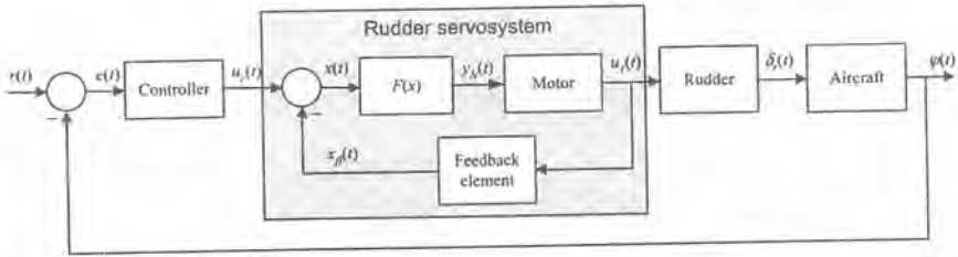
Figure 7.5: Block diagram of an airplane course control system.
