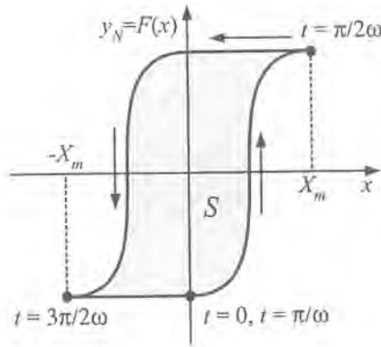
Figure 3.10: Multi-valued nonlinear static characteristic (hysteresis type).
