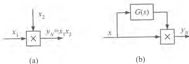
Figure 1.31: Element for multiplication.
