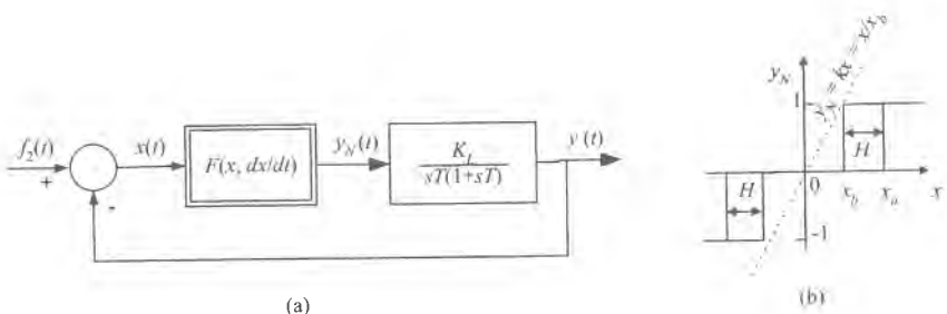
Figure 2.35: Block diagram of nonlinear system (a) and static characteristic of nonlinear element (b).
