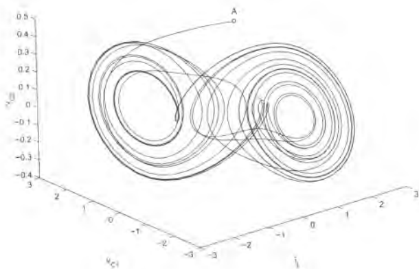
Figure 1.9: State trajectory ( i_L, v_{C1}, v_{C2} ) of Chua circuit in chaos.
