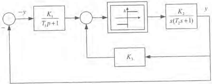
Figure 8.7: Block diagram of a nonlinear servo system.
