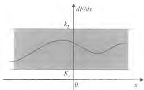
Figure 2.42: The gradient of nonlinear characteristic must be limited.
