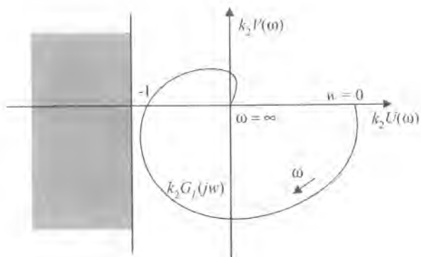
Figure 2.41: Prohibited region for frequency characteristic of linear stable part k_2 G_L(j\omega) .
