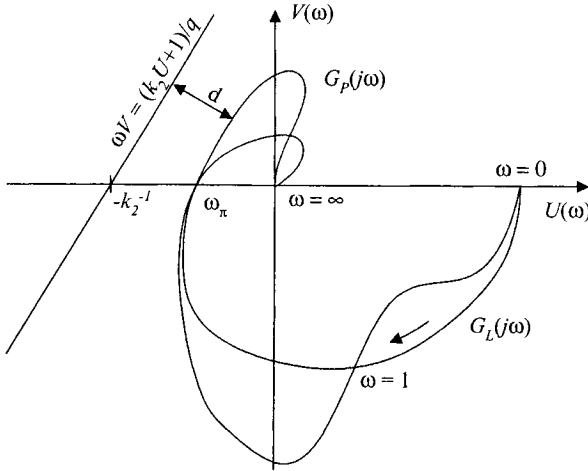
Figure 2.22: Popov line doesn't intersect Popov plot—graphical condition of absolute stability.
