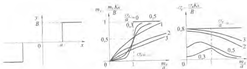
Figure 3.17: Normalized K_M and K_S for the nonlinearity of the type three-position relay without hysteresis.
