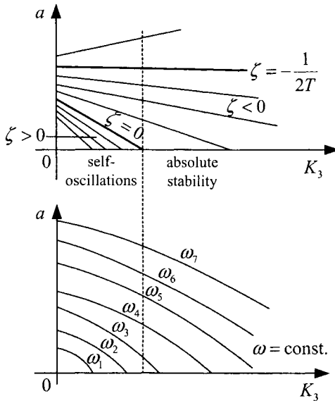
Figure 8.8: Diagram of performance indicators for transient response of a nonlinear servo system—Example 8.4.
