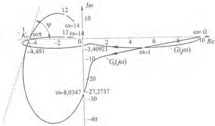
Figure 2.29: Graphical solution of Example 2.19.
