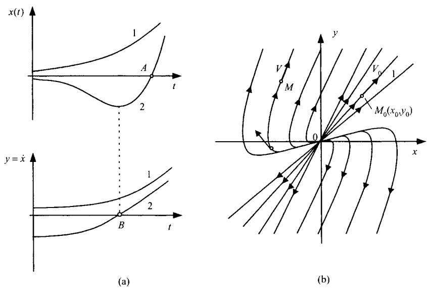
Figure 5.6: Possible phase trajectories (a) and phase portrait (b) of linear system with singular point of type unstable node.
