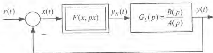
Figure 7.1: Block diagram of nonlinear control system with nearly constant reference signal r(t) .
