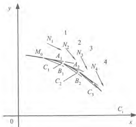
Figure 5.11: Construction of phase trajectories by isocline method.
