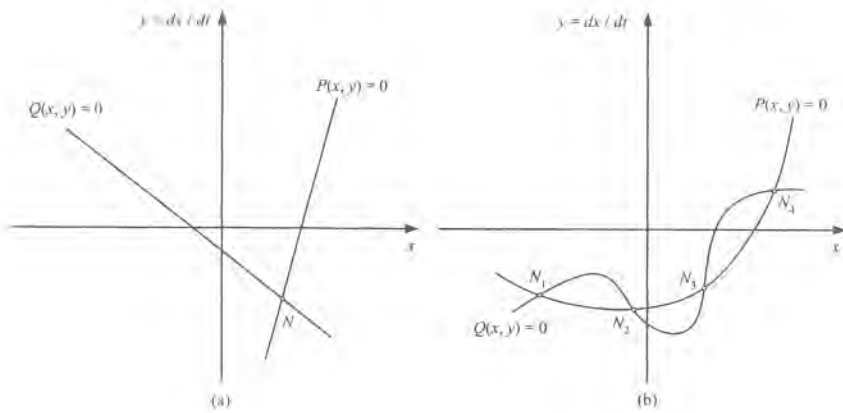
Figure 5.10: Singular point N of linear system (a), and singular points of nonlinear system (b).
