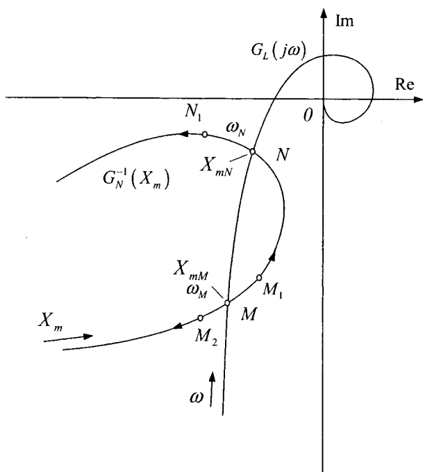
Figure 6.3: Goldfarb method of finding parameters of self-oscillations.
