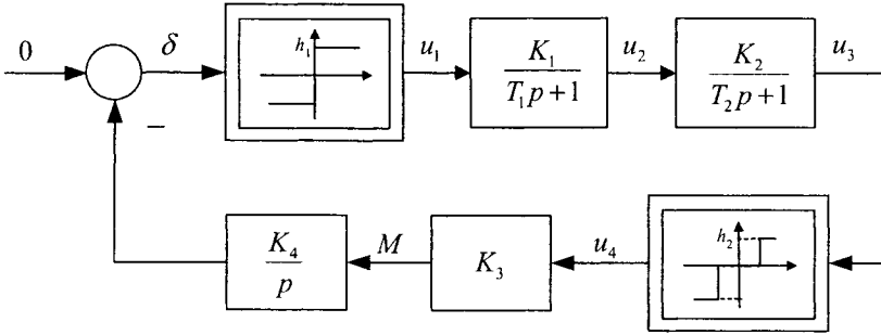
Figure 8.2: Block diagram of a nonlinear servo system in stabilization mode.
