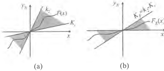
Figure 2.27: (a) Reduced allowable sector [K_r, k_2] for nonlinear characteristic F(x) , (b) Corresponding allowed sector [0, K_F] for equivalent nonlinear characteristic F_E(x) .
