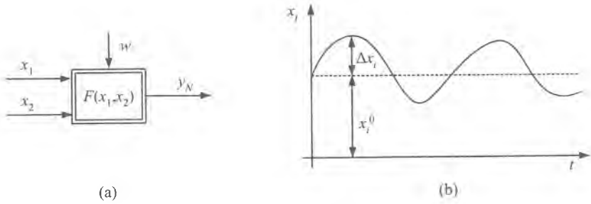
Figure 3.3: Nonlinear system with three inputs (excitations) and one output (response).
