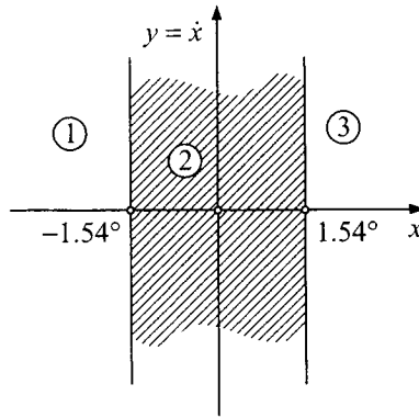
Figure 5.22: Sheets in phase plane.
