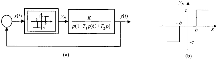
Figure 6.7: Block diagram of unforced closed-loop control system and nonlinear static characteristic of nonlinear element.
