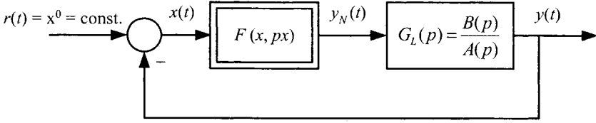
Figure 6.13: Block diagram of a forced nonlinear control system.
