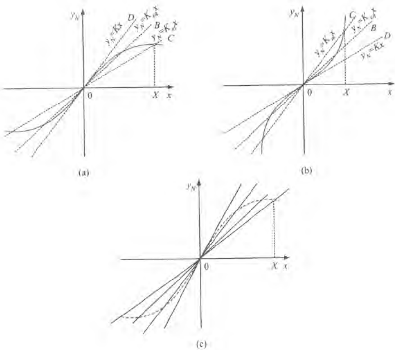
Figure 3.6: Linearization of static characteristics with straight lines.
