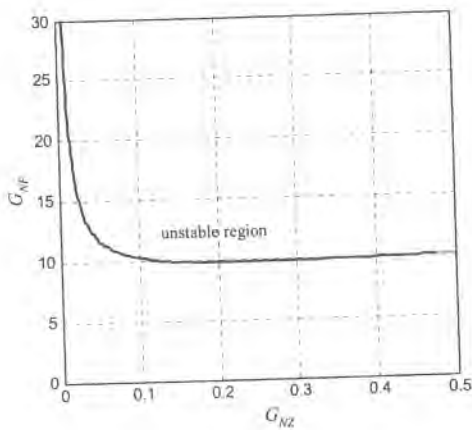
Figure 9.24: Stability boundary G_{NF} = f(G_{NZ}) .
