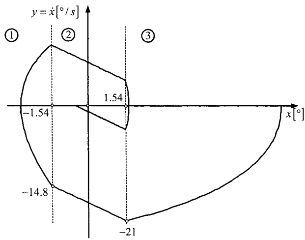
Figure 5.23: Phase trajectory obtained by method of adjoint solutions.
