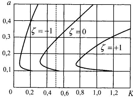
Figure 8.6: Diagram of performance indicators of a servo system from Example 8.3.
