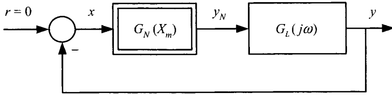
Figure 6.2: Block diagram of an unforced nonlinear control system, linearized by harmonic linearization.
