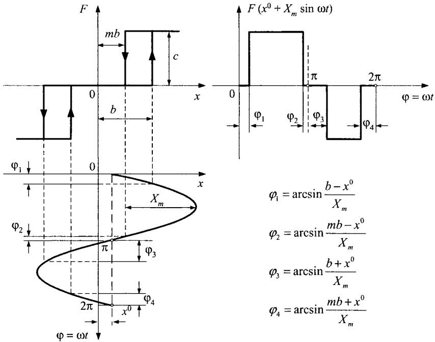
Figure 6.14: Input and output signals of a three-position relay with hysteresis.
