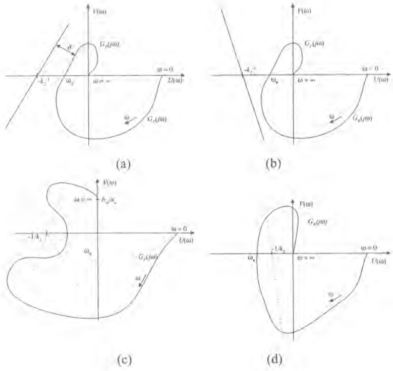
Figure 2.23: Absolute stable ((a) and (b)) and unstable ((c) and (d)) equilibrium states.
