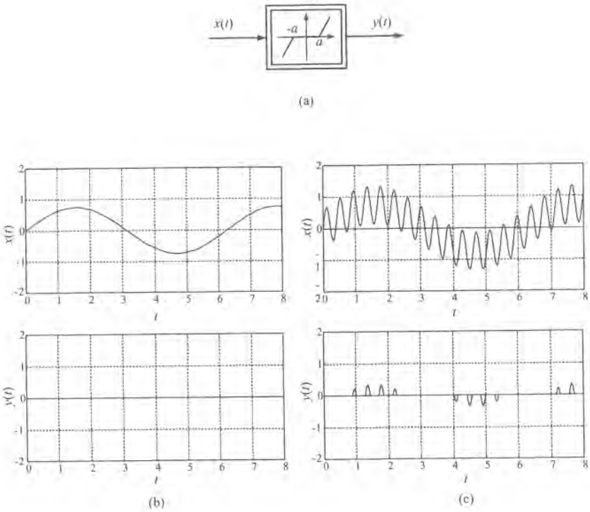
Figure 4.1: (a) Static characteristic of nonlinear element dead zone, (b) harmonic signal (information carrier), and (c) superimposed dither at the input and the signal of the output of the dead zone element.
