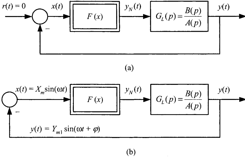
Figure 6.1: (a) Block diagram of an unforced nonlinear control system, (b) established monoharmonic (self-) oscillations.
