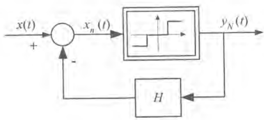
Figure 2.36: Equivalent structure for multi-valued nonlinear characteristic of three-position relay with hysteresis (Fig. 2.35b).
