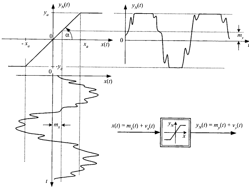
Figure 3.14: Noise corrupted excitation and response of a saturation nonlinearity.
