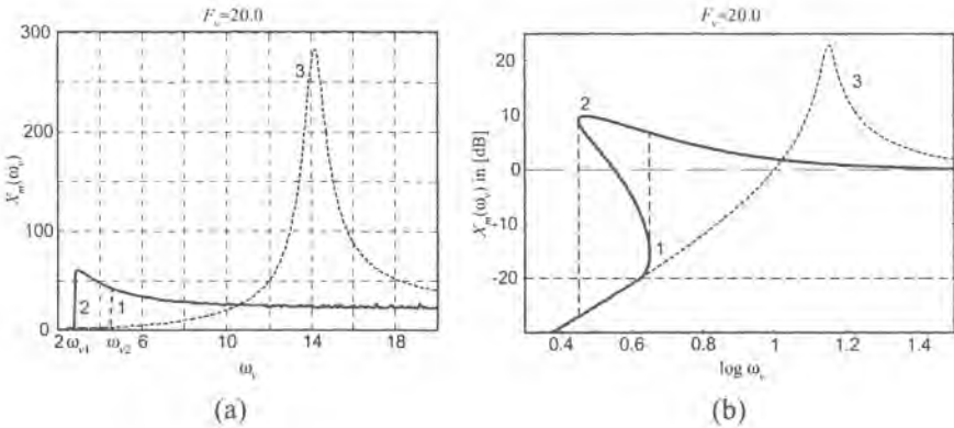
Figure 6.33: The frequency characteristic X_m(\omega_v) : (a) obtained by simulation and (b) determined analytically. Legend: 1 – frequency increases, 2 – frequency decreases, 3 – linear system frequency response.
