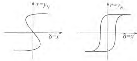
Figure 1.13: Static multi-valued nonlinear characteristics of course unstable ships.
