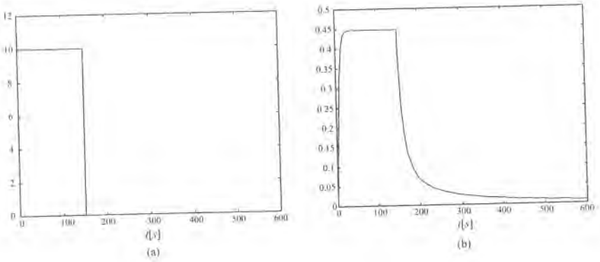
Figure 1.5: Thrust (a) and velocity (b) of an underwater vehicle.
