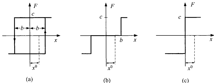
Figure 6.15: Relay characteristics: (a) with hysteresis, (b) with dead zone, and (c) ideal two-position relay.
