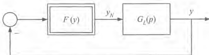
Figure 2.17: Structure of unforced nonlinear system.
