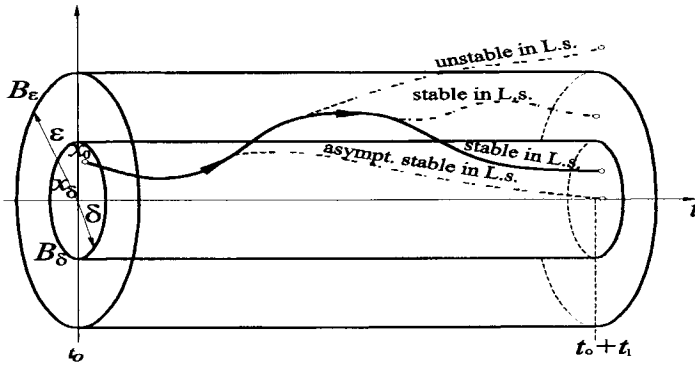
Figure 2.7: Behavior of stable and unstable state trajectory with time.
