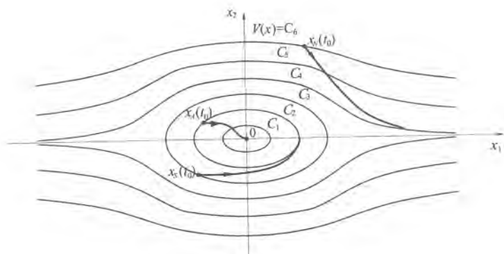
Figure 2.11: Example of a possible Lyapunov plane for a second-order system.
