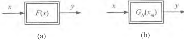
Figure 3.8: Nonlinear block (a) and block with describing function (b).
