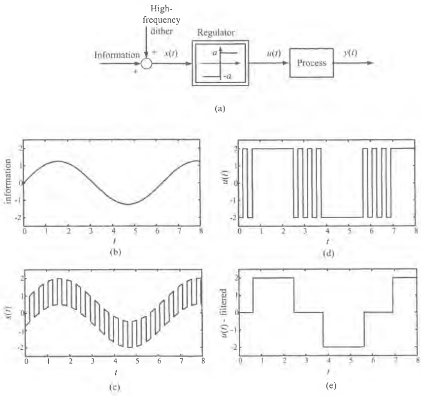
Figure 4.2: (a) Block diagram of two-position control of process, (b) excitation at the input of two-position control without dither, (c) excitation with superimposed rectangular dither signal, (d) output of the two-position regulator, (e) filtered signal as “seen” by the process.
