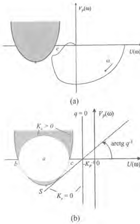
Figure 2.28: Prohibited region for modified Popov plot.
