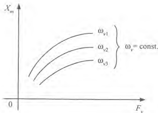
Figure 6.18: The amplitudes of oscillations at the input to the nonlinear element depend on the amplitude and frequency of the exciting harmonic signal to the nonlinear closed-loop control system.
