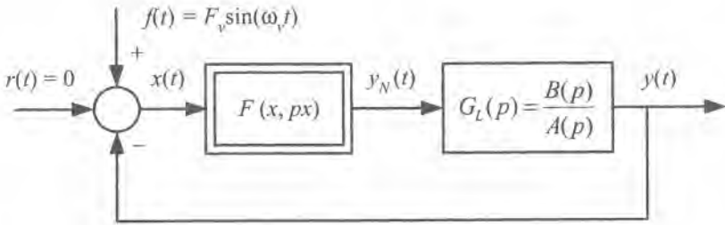
Figure 6.17: Block diagram of a nonlinear closed-loop control system subject to harmonic signal.
