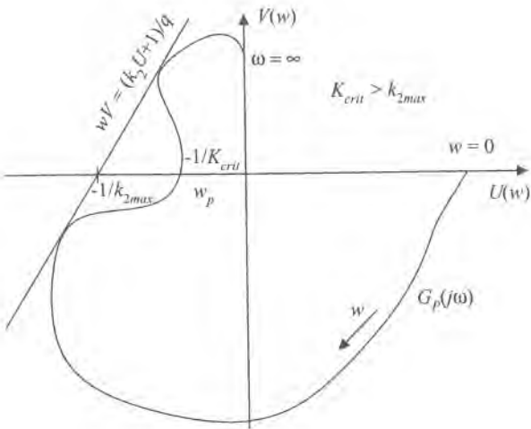
Figure 2.24: Determining of maximum allowable gain.
