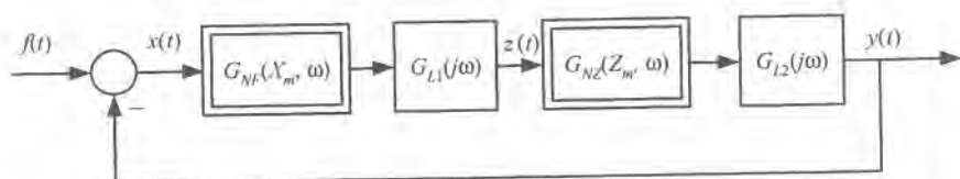
Figure 9.18: The structure of a nonlinear system with fuzzy regulator.
