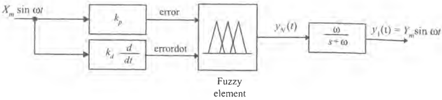
Figure 9.14: The circuit scheme for experimental determination of the describing function.
