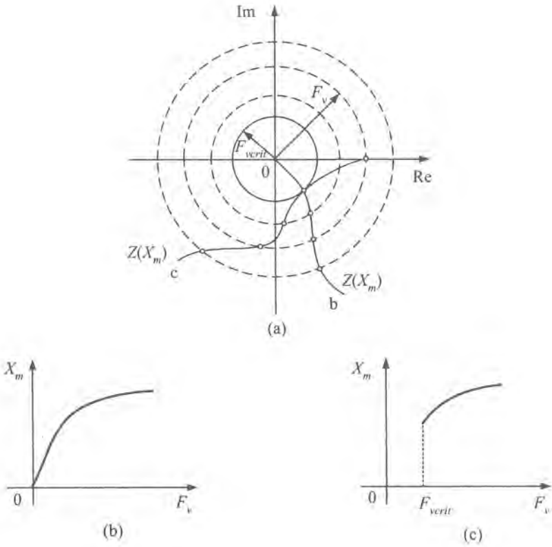
Figure 6.21: Graphical procedure of finding how the amplitudes of forced oscillations depend on excitation amplitude, F_v : (a) Z(X_m) for F_{vcrit} = 0 and F_v > 0 , (b) X_m = X_m(F_v) for F_{vcrit} = 0 , and (c) X_m = X_m(F_v) for F_{vcrit} > 0 .
