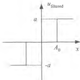
Figure 4.3: Equivalent nonlinearity for two-position controller with superimposed rectangular dither signal.
