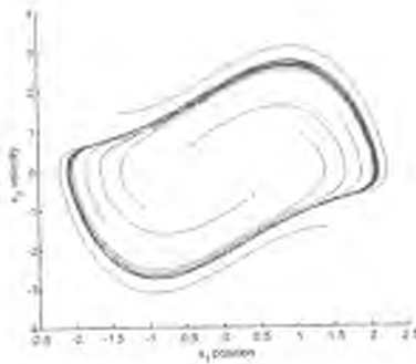
Figure 2.3: Phase trajectories of Van der Pol equation.
