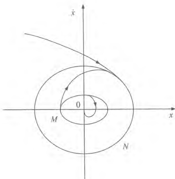
Figure 6.4: Phase trajectories of system which has unstable self-oscillations (limit cycle is smaller ellipse) and stable self-oscillations (limit cycle is larger ellipse).
