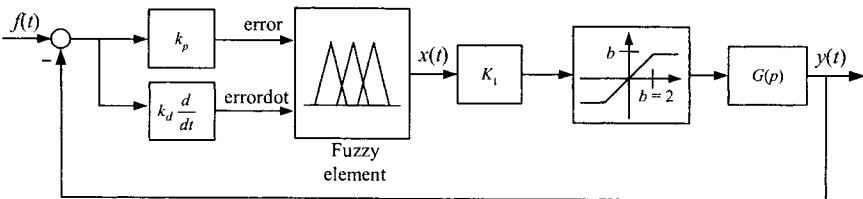
Figure 9.26: System with fuzzy regulator (Example 9.4).
