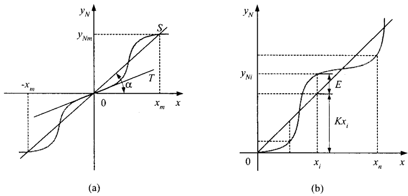
Figure 3.2: Linearization of smooth nonlinear static characteristic by the secant line.
