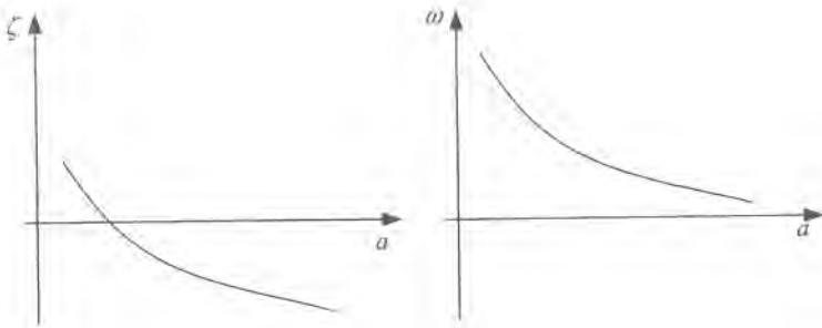
Figure 8.3: The dependence of 'damping' and 'frequency' on the amplitude of oscillations.
