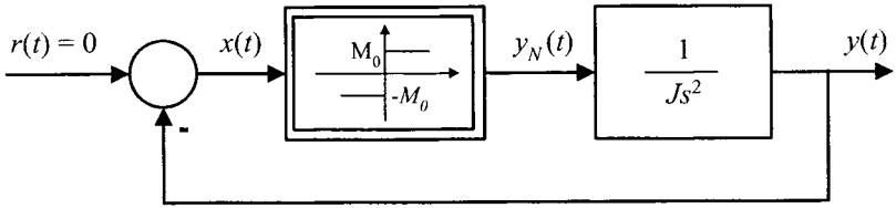
Figure 5.18: Block diagram of nonlinear system.
