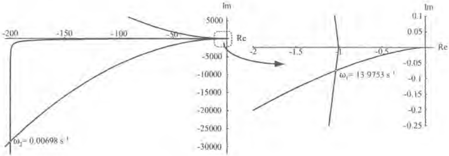
Figure 6.32: Frequency characteristic of linear part of the system G_L(j\omega_v) and envelope A .
