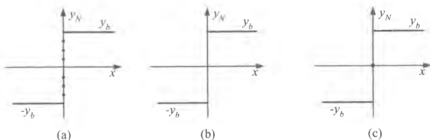
Figure 1.21: Ideal static characteristics of a two-position relay.
