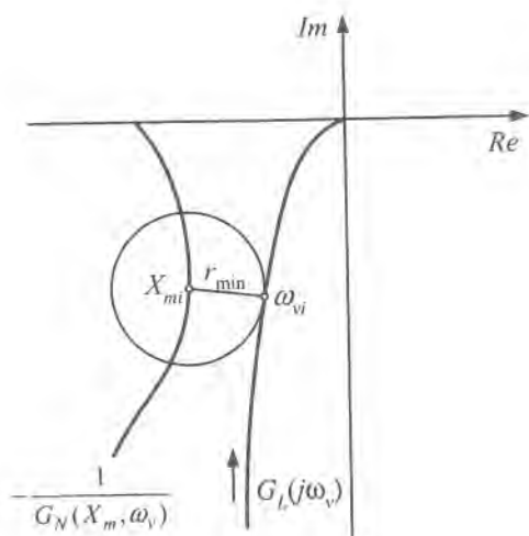
Figure 6.28: The determination of F_{vcrit} for given value of \omega_v .
