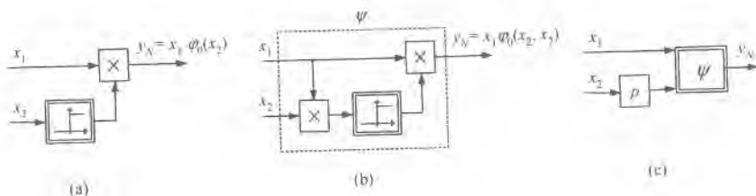
Figure 1.34: Various realizations of special nonlinear elements.
