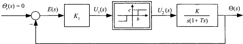
Figure 5.21: Block diagram of a servo system.
