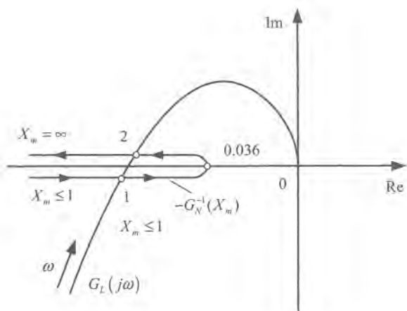
Figure 6.8: Plot of negative inverse describing function and frequency characteristic of linear part of closed-loop control system.
