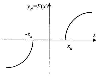
Figure 2.21: Nonlinear static characteristic of dead zone.
