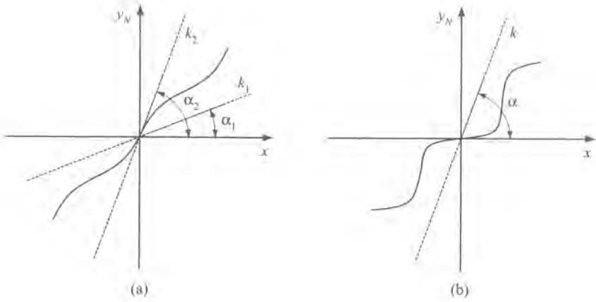
Figure 1.35: Nonlinear functions of class [k_1, k_2] (a) and of class [0, k] (b).
