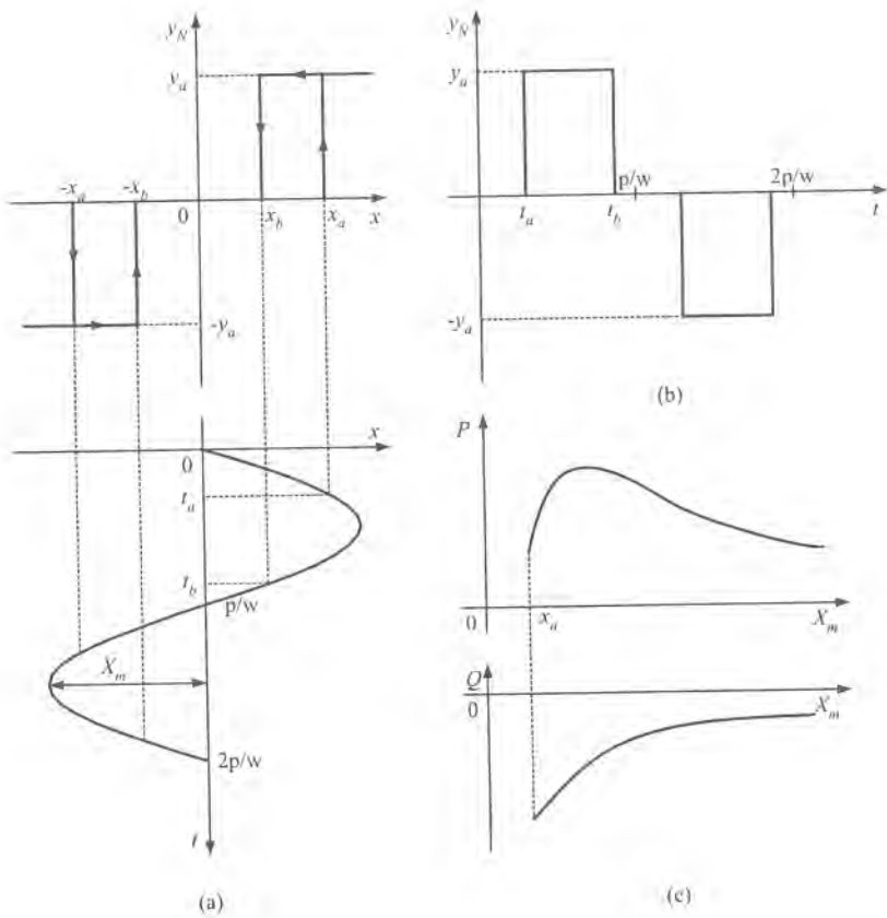
Figure 3.11: Static characteristics with input (a) and output (b), as well as with real and imaginary part (c) of the describing function of the three-position relay with hysteresis.
