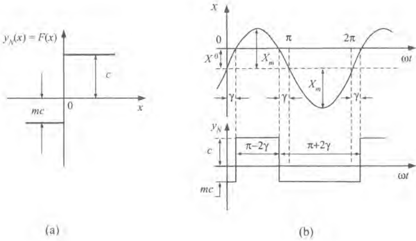
Figure 6.11: (a) Asymmetrical static characteristic of nonlinear element, (b) input and output signal of an asymmetrical nonlinearity.
