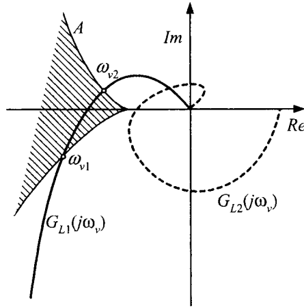
Figure 6.30: Qualitative display of frequency area where resonance jump is possible.
