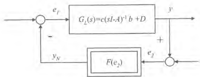
Figure 2.16: Structure of nonlinear systems in the problems of analysis of absolute stability.
