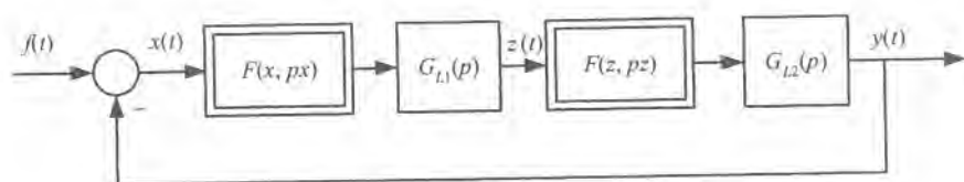
Figure 9.18: The structure of a nonlinear system with fuzzy regulator.
