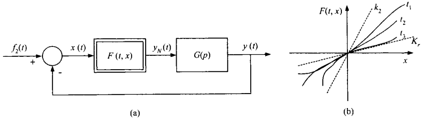
Figure 2.32: Structure of nonlinear system and static characteristics of nonlinear part of system which vary with time, but never come out of sector [K_r, k_2] .
