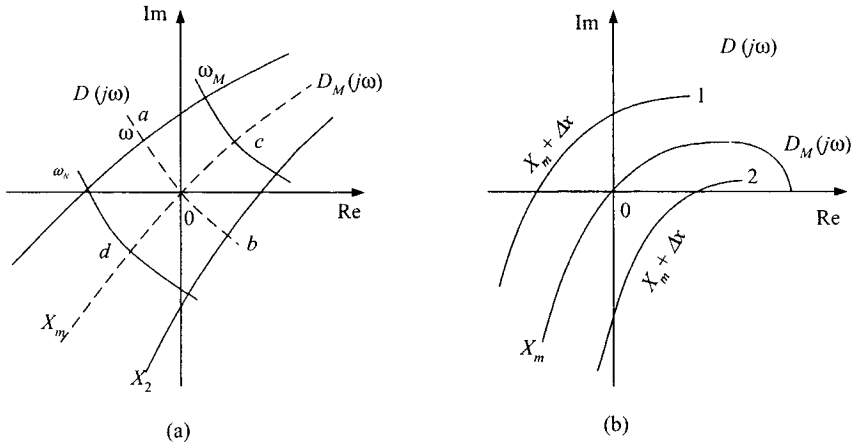
Figure 6.6: Mikhailov plots.
