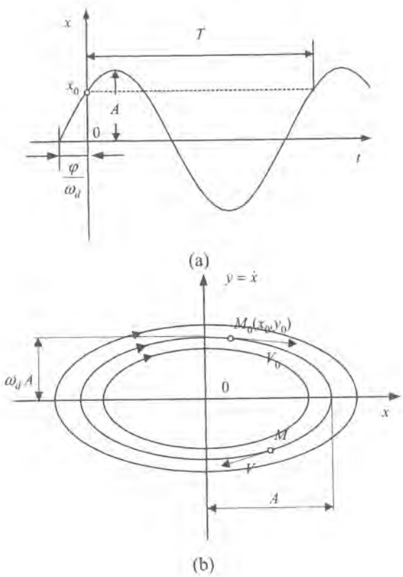
Figure 5.2: State behavior of linear system (a) and phase portrait for case of singular point of the type center (b).
