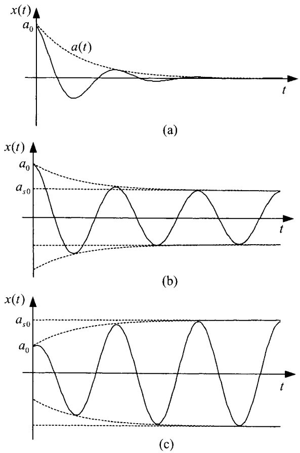
Figure 8.5: Transient responses of a nonlinear control system: (a) damped oscillatory, (b) damped oscillatory ending in self-oscillations, (c) increasing oscillatory ending in self-oscillations
