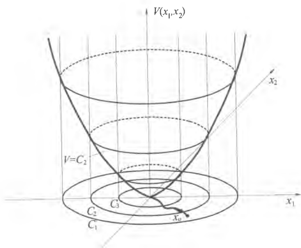
Figure 2.10: Possible form of Lyapunov function for a second-order system.
