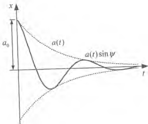
Figure 8.1: Damped oscillatory transient response of a nonlinear control system.
