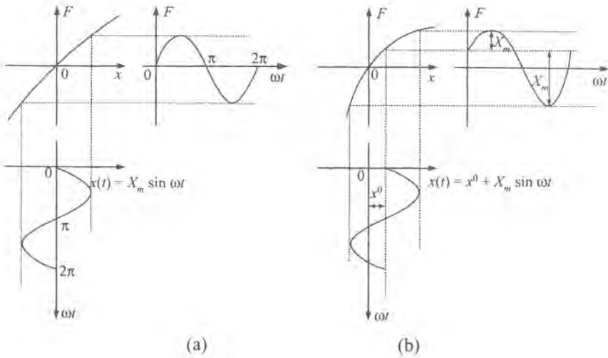
Figure 6.10: Effect of asymmetrical static characteristic of a nonlinear element.
