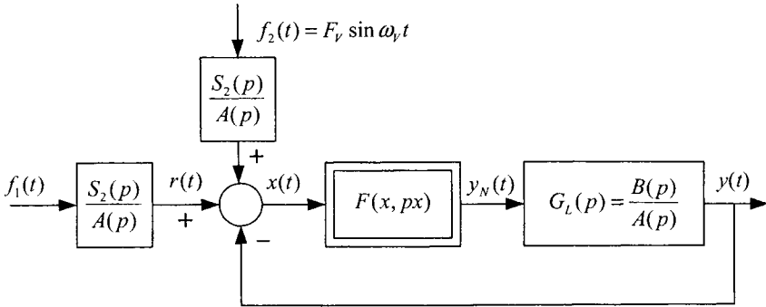
Figure 7.6: Block diagram of a nonlinear closed-loop control system in tracking mode of operation.
