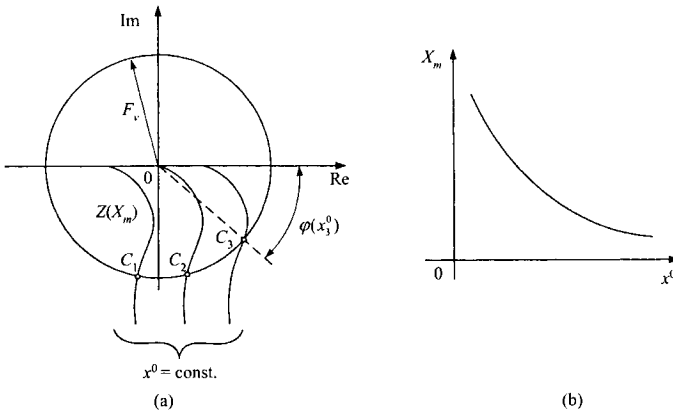
Figure 6.25: Graphical procedure to determine the parameters of asymmetrical forced oscillations: (a) graphical solution for X_m given by various x^0 = \text{const.} , (b) plot of X_m = X_m(x^0) obtained from procedure in (a).
