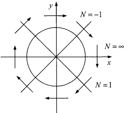
Figure 5.20: Phase trajectories by isocline method.
