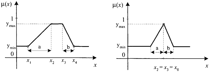
Figure 9.5: Common membership function in the shape of trapezoid and triangle.
