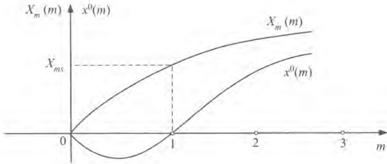
Figure 6.12: The relation between X_m(m) and x^0(m) according to expressions (6.89) and (6.84).
