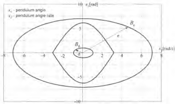
Figure 2.6: State trajectory of a pendulum.
