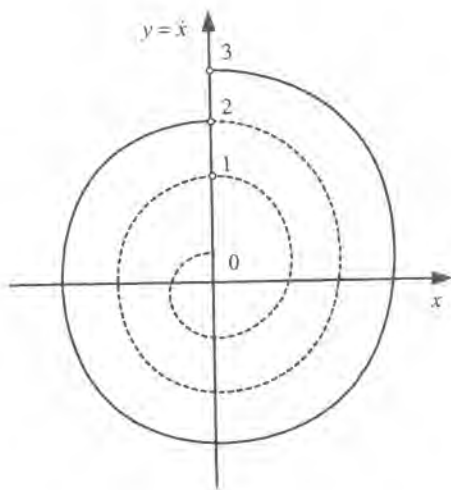
Figure 5.13: Phase trajectory of a nonlinear system.
