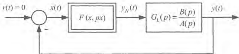
Figure 6.9: Block diagram of unforced nonlinear closed-loop control system.
