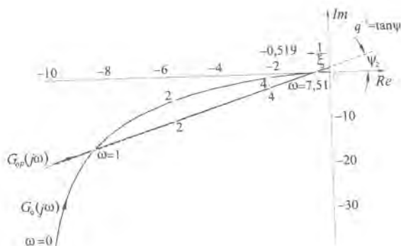
Figure 2.31: Graphical solution of Example 2.21.
