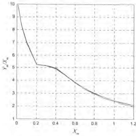
Figure 9.23: Describing function of fuzzy regulator.
