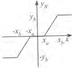
Figure 1.18: Static characteristic of saturation with dead zone.
