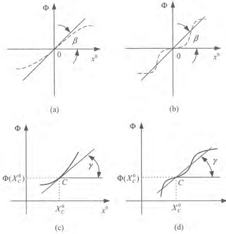
Figure 7.4: Linearization of various smoothed static characteristics.
