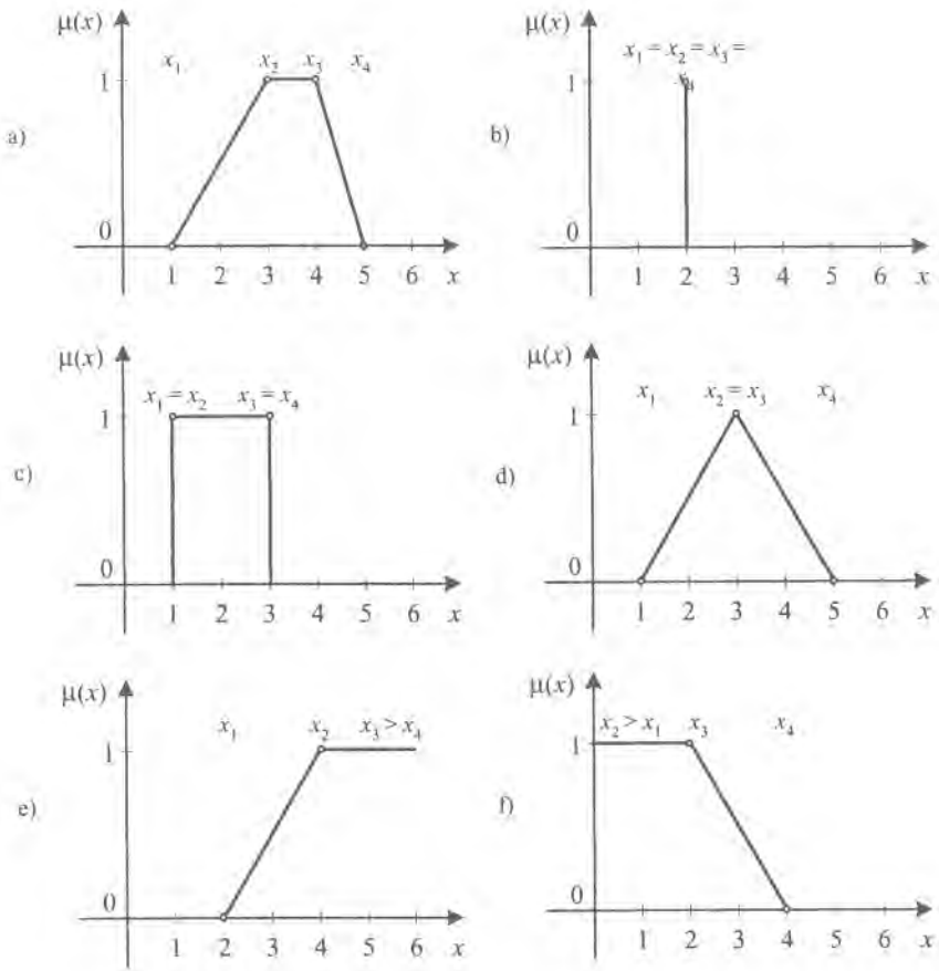
Figure 9.4: Membership functions in the shape of trapezoid and its derivations.
