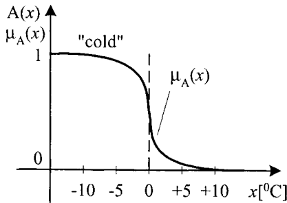
Figure 9.2: Fuzzy set A membership function.
