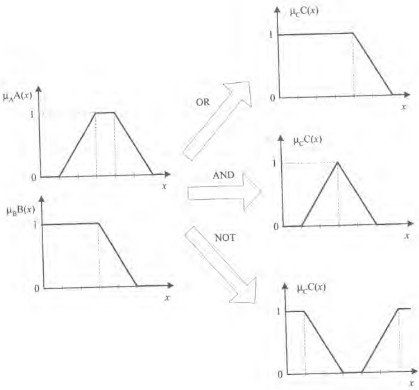
Figure 9.7: Basic procedures on fuzzy sets.
