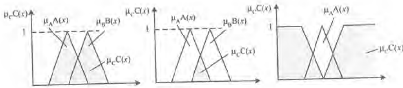
Figure 9.8: Basic procedures on triangle fuzzy sets.
