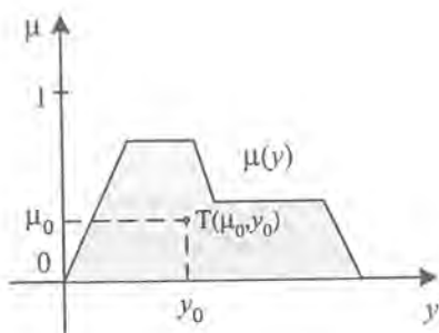
Figure 9.12: Calculating output value by method of gravity center.
