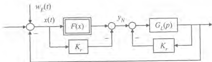
Figure 2.19: Equivalent structure of nonlinear system in the case of unstable linear part.
