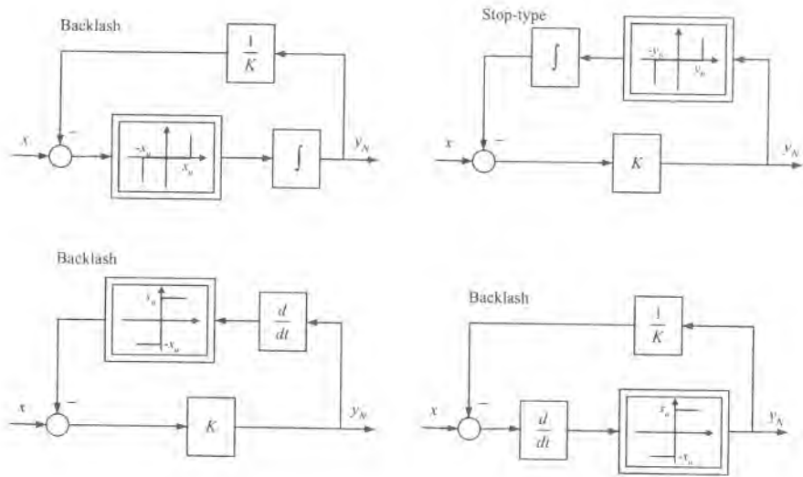
Figure 1.29: Possible realizations of nonlinear characteristics of backlash and stop-type element.
