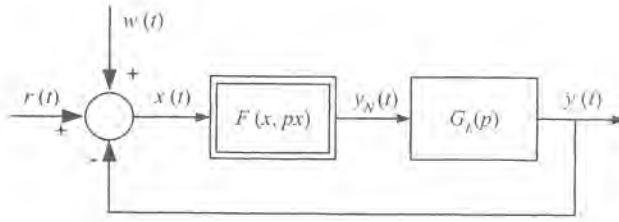
Figure 1.2: Simplified block diagram of a nonlinear system.
