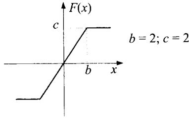
Figure 6.31: Static characteristic of the nonlinearity in Example 6.7.
