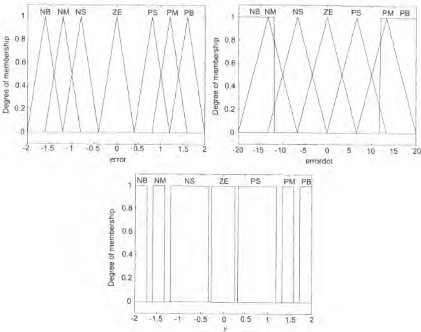
Figure 9.15: Membership functions of the fuzzy element inputs 'error' and 'error-dot' and fuzzy element output y = y_N .
