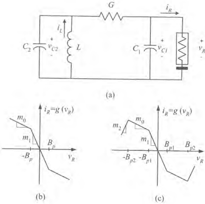
Figure 1.8: Electrical scheme of Chua circuit (a), nonlinear characteristic of the resistor (b), modified resistor characteristic (c).
