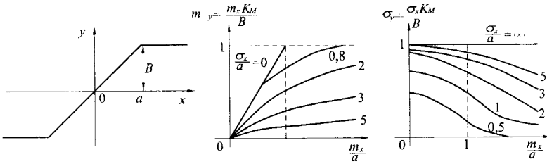
Figure 3.16: Normalized K_M and K_S for the nonlinearity of the type saturation.
