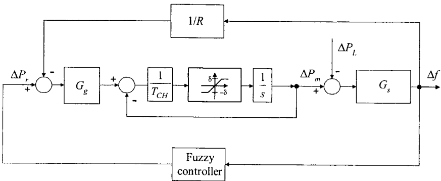
Figure 9.20: Power system secondary-load frequency control model (Example 9.3).
