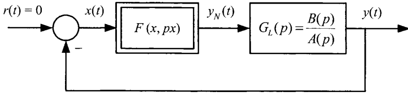
Figure 6.5: Block diagram of an unforced nonlinear control system.
