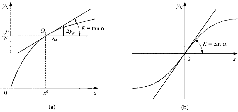
Figure 3.1: Linearization of smooth nonlinear static characteristics by the tangent line.
