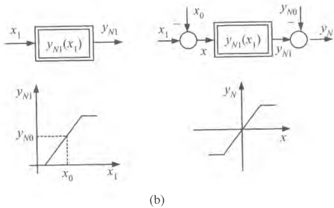
Figure 1.15: Asymmetrical characteristic becomes even (a) and odd (b) symmetrical.
