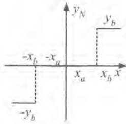
Figure 1.20: Static characteristic of a three-position relay without hysteresis.
