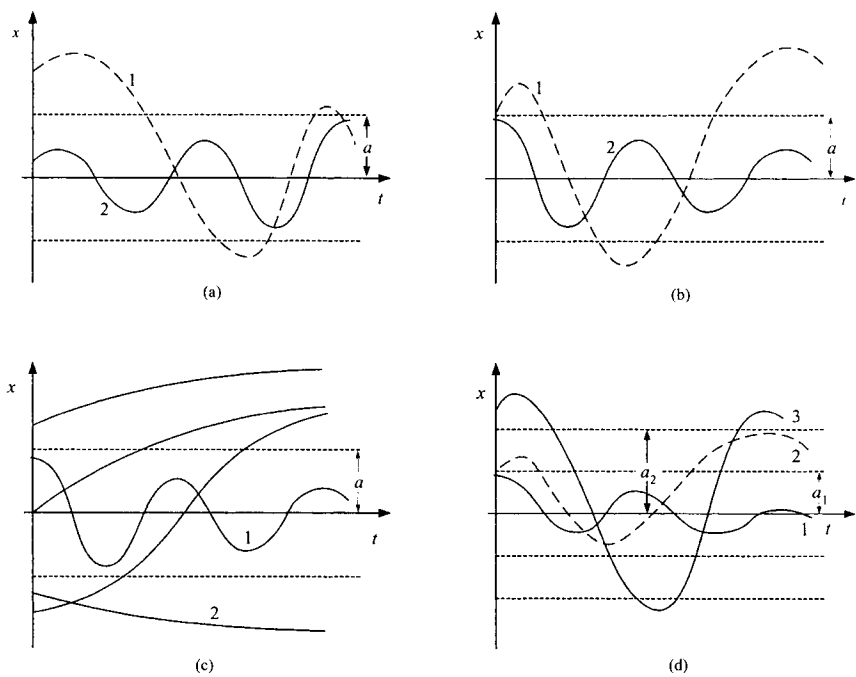
Figure 5.8: Possible forms of solution of an unforced nonlinear system.
