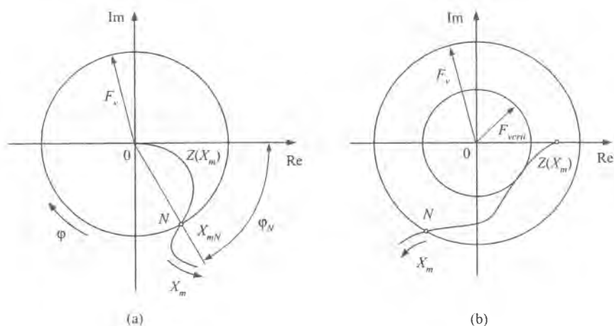
Figure 6.19: Graphical procedure of determining the parameters (amplitude and frequency) of forced oscillations, (a) for F_{vcrit} = 0 , (b) for F_{vcrit} > 0 .
