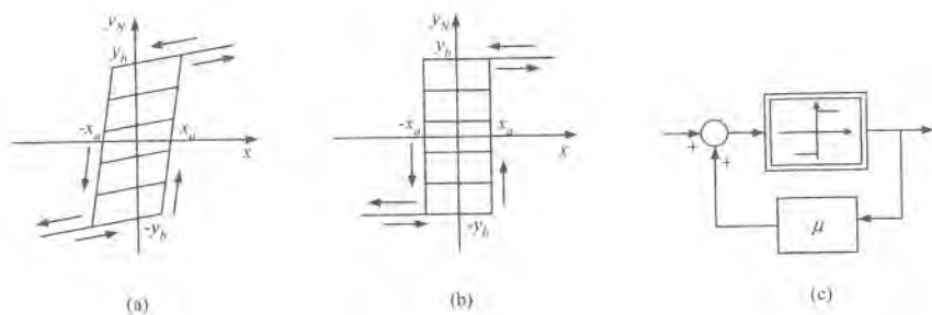
Figure 1.30: Static characteristic of a magnetic hysteresis.
