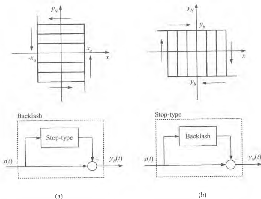
Figure 1.28: Nonlinear characteristics of backlash (a) and stop-type element (b) at high gains.
