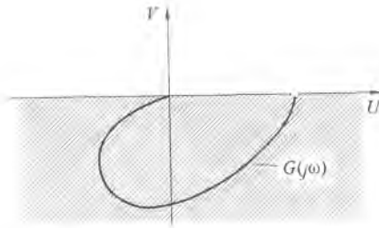
Figure 2.34: Frequency characteristic of stable linear part G_L(j\omega) = G(j\omega) .
