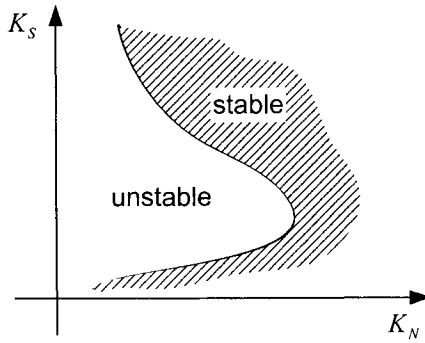
Figure 7.9: Stability region in parametric plane.
