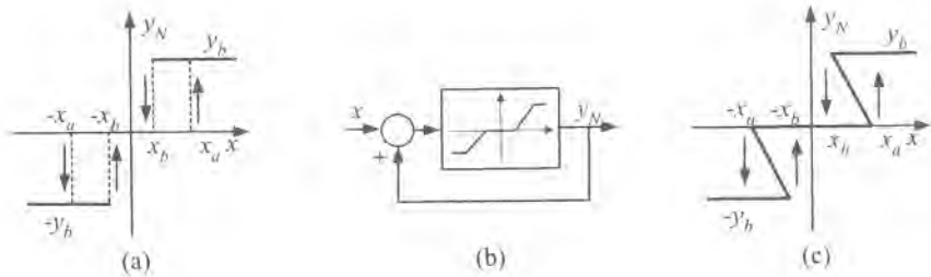
Figure 1.23: Static characteristics of a three-position relay with hysteresis.
