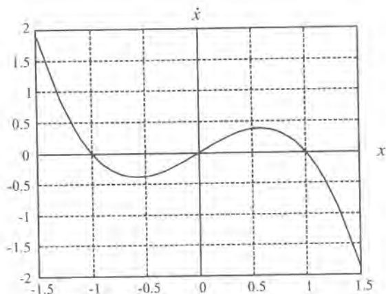
Figure 1.11: State trajectory of the system \dot{x} = x - x^3 .
