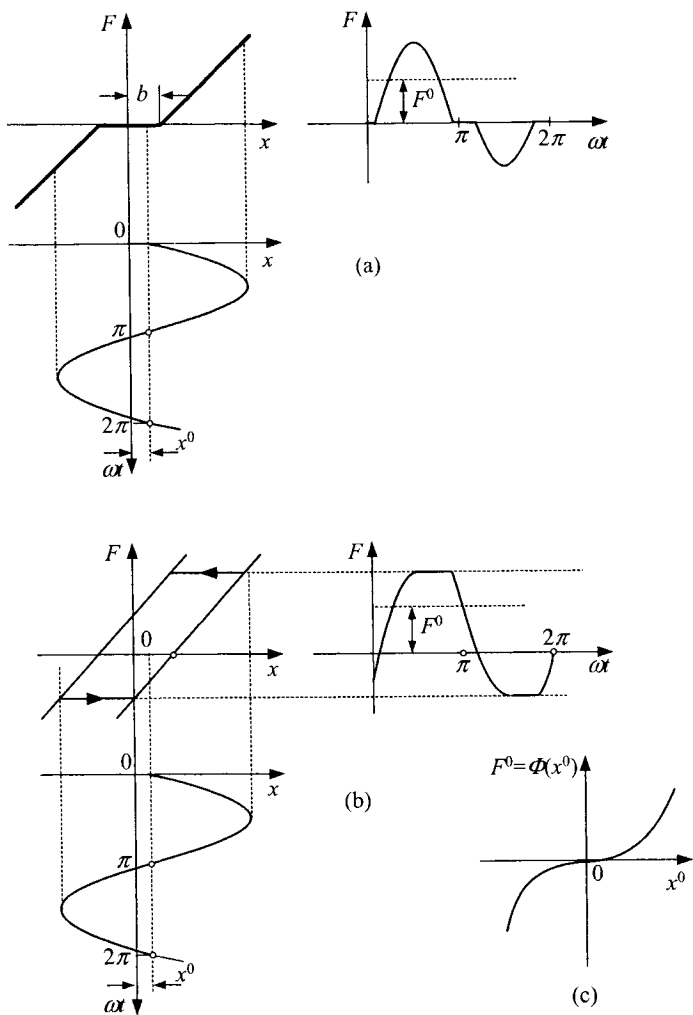
Figure 7.3: Effects which harmonic inputs produce on nonlinear element of type dead zone (a), of type backlash (b) and smoothed static characteristic of nonlinearity (c).
