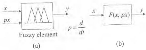
Figure 9.13: Description of the fuzzy logic element with SISO nonlinear element.
