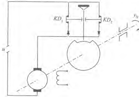
Figure 1.27: Schematic of ship's rudder driven by an electromotor.
