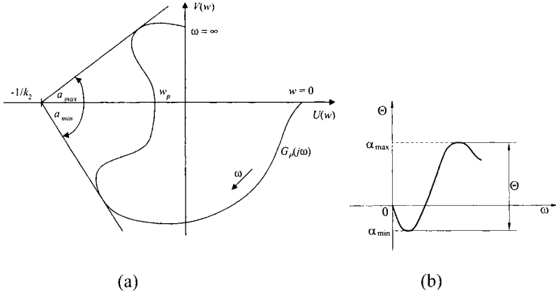
Figure 2.26: Graphical interpretation \alpha_{\max} and \alpha_{\min} in the region 0 < \omega < \infty .
