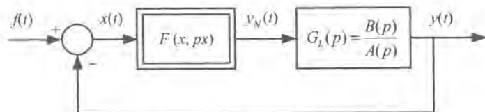
Figure 6.26: Block diagram of a forced system.
