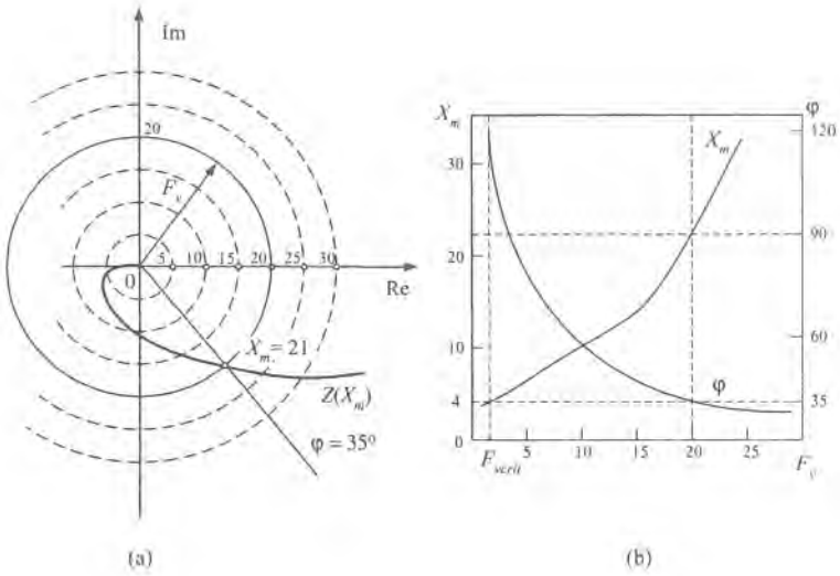
Figure 6.24: Graphical display of solving the problem of forced oscillations for Example 6.6.
