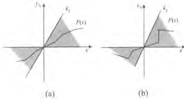
Figure 2.40: Example of allowed (a) and prohibited (b) nonlinear characteristics.
