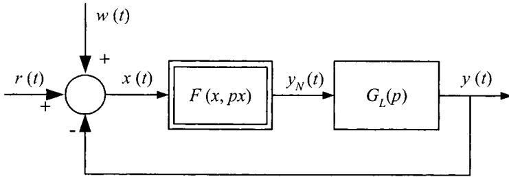
Figure 2.18: Basic structure of a nonlinear system for analysis of absolute stability with external signals r(t) and w(t) .
