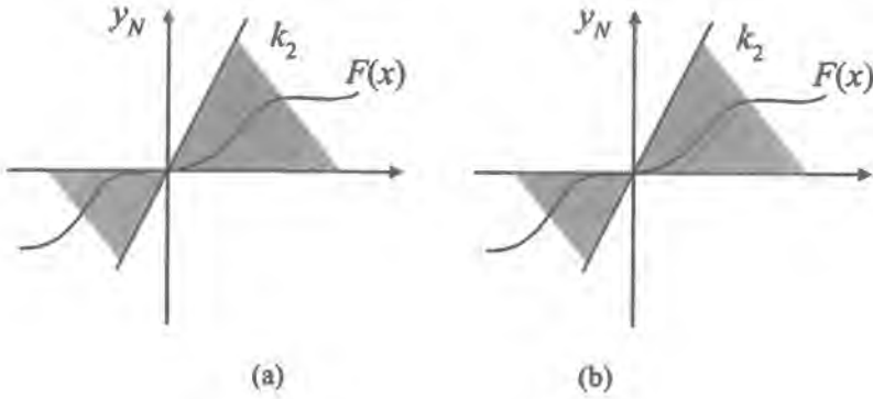
Figure 2.20: Nonlinear characteristic F(x) of (a) class [0, k_2] and (b) class [K_r, k_2] .
