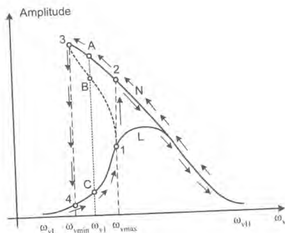
Figure 1.6: Frequency characteristics of linear (L) and nonlinear (N) system.
