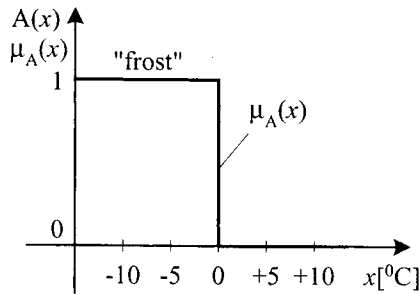
Figure 9.1: Crisp set A membership function \mu_A .
