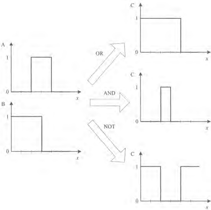
Figure 9.6: Basic procedures on crisp sets.
