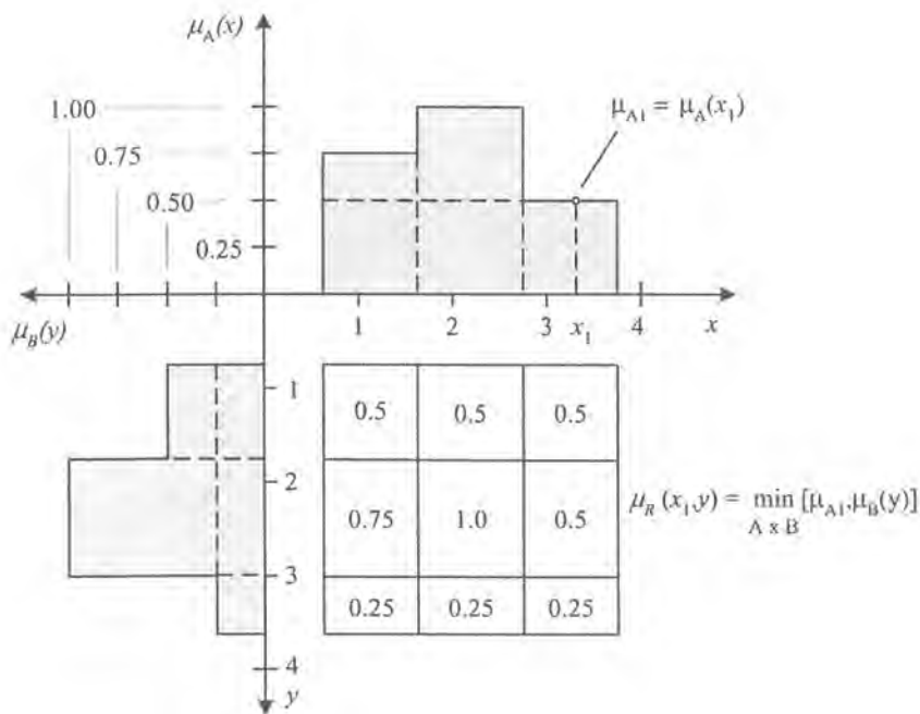
Figure 9.9: An example of membership function defining for the given fuzzy relation.
