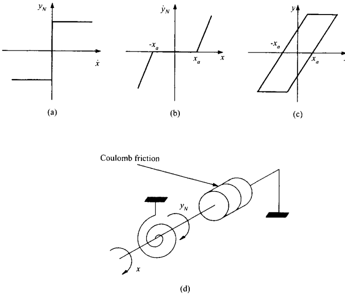
Figure 1.25: Static characteristics of Coulomb friction.
