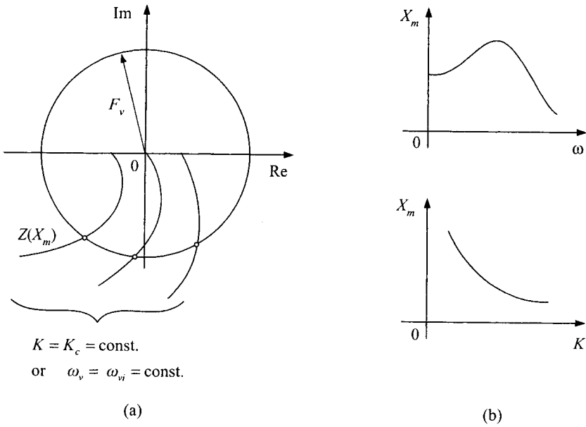
Figure 6.20: Graphical procedure to determine how the parameters of forced oscillations depend on exciting frequency or some other parameter of control system: (a) Z(X_m) for various K = \text{const.} or \omega_v = \text{const.} (b) X_m = X_m(\omega_v) and X_m = X_m(K) according to graphical solution of (6.150).
