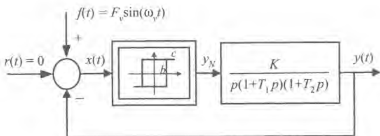
Figure 6.23: Block diagram of a nonlinear closed-loop control system in stabilization mode.
