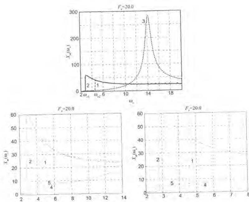
Figure 9.27: Frequency response of the system in Example 9.4. Legend: 1—increasing frequency (without fuzzy regulator); 2—decreasing frequency (without fuzzy regulator); 3—linear system; 4—increasing frequency (with fuzzy regulator); 5—decreasing frequency (with fuzzy regulator).
