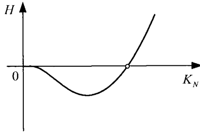
Figure 7.8: The stability boundary of a nonlinear system—Example 7.2.
