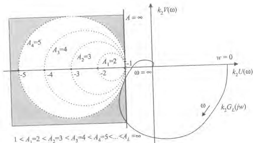
Figure 2.43: Circle criterion of absolute stability in the plane [k_2U(\omega), k_2V(\omega)] .
