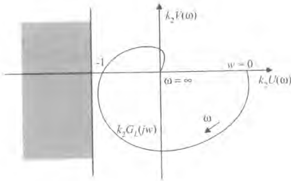
Figure 2.33: Example of absolute stable time-varying nonlinear system.
