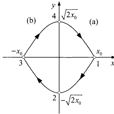
Figure 5.19: Phase trajectory.
