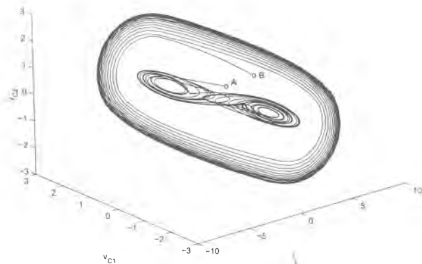
Figure 1.10: State trajectories ( i_L, v_{C1}, v_{C2} ) of Chua circuit with modified nonlinear resistor characteristics.
