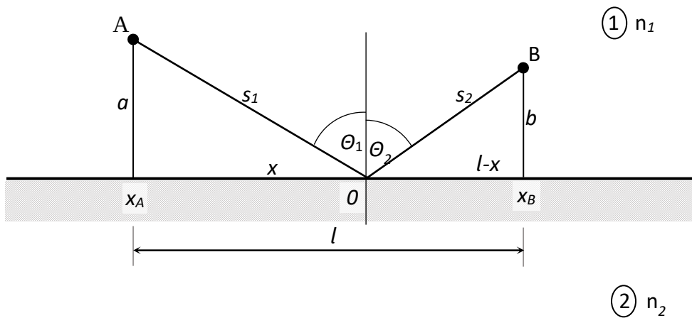
Figure 3: Reflection of the light ray in rectangular coordinates
