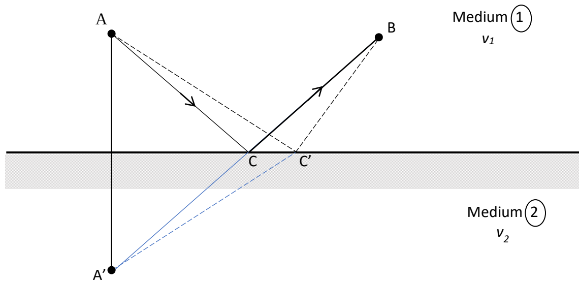
Figure 1: Reflection of the light ray
