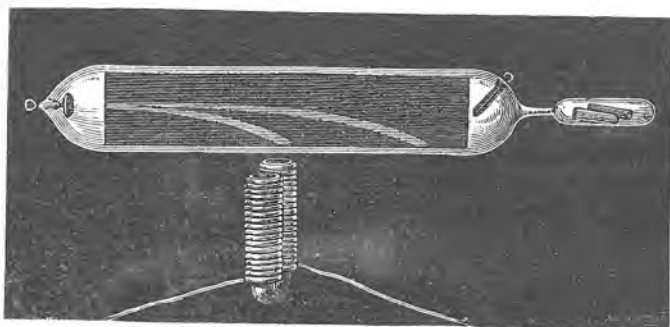
Sl. 218. Magnet otklanja katodne zrake.
